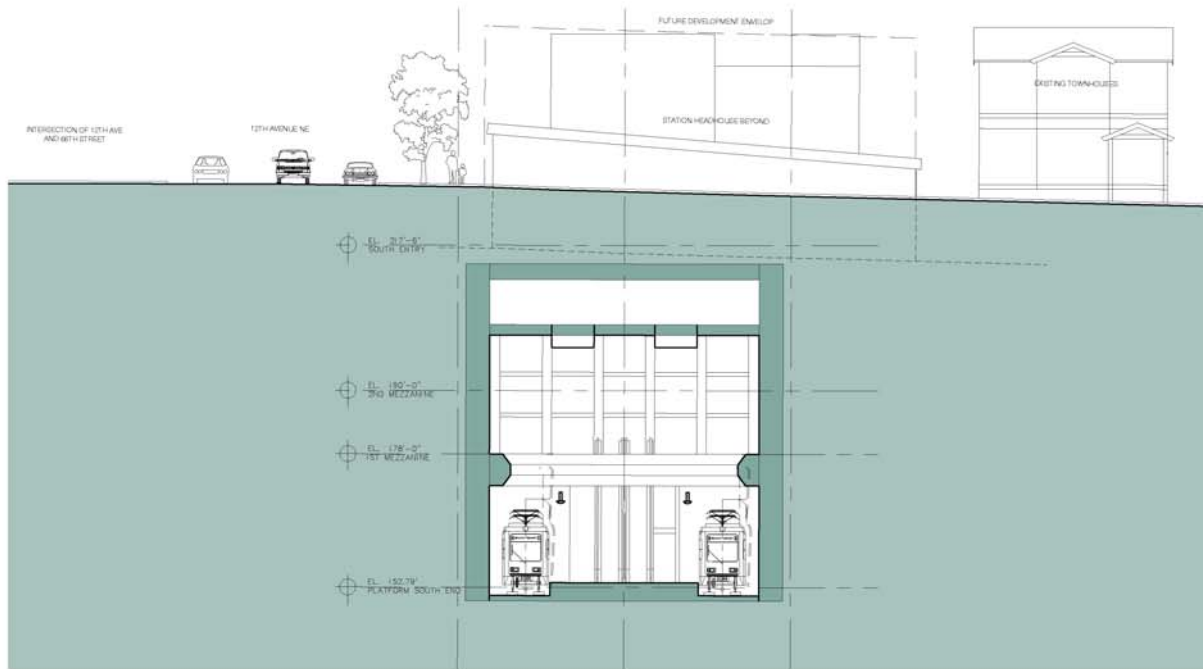
SECTION AT PLATFORM CENTER
