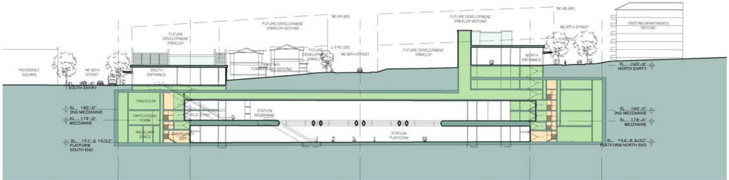
LONGITUDINAL SECTION (FACING WEST)
