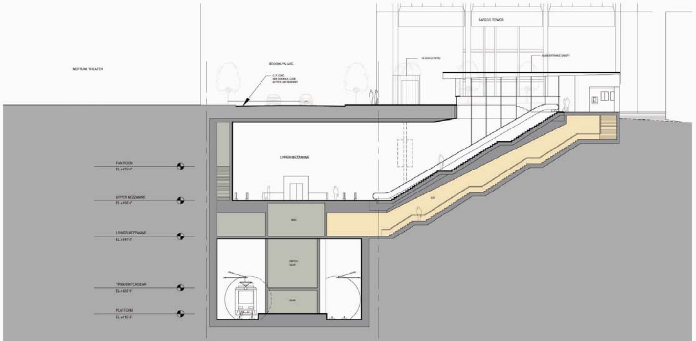
SECTION, NORTH ENTRANCE
