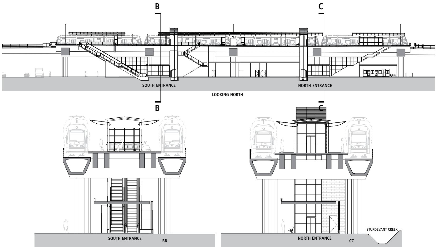
Cross sections
