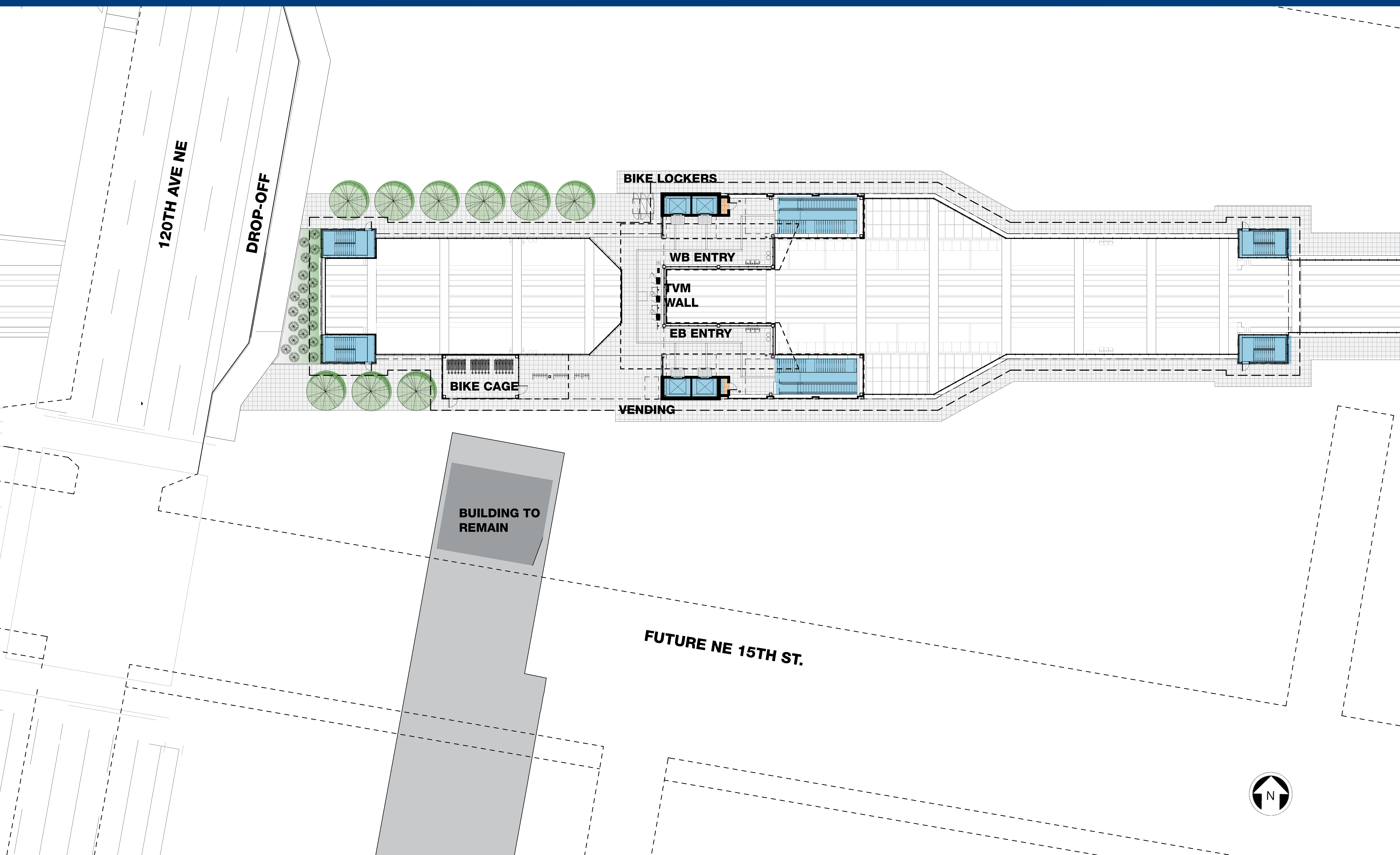
Interim station site plan
