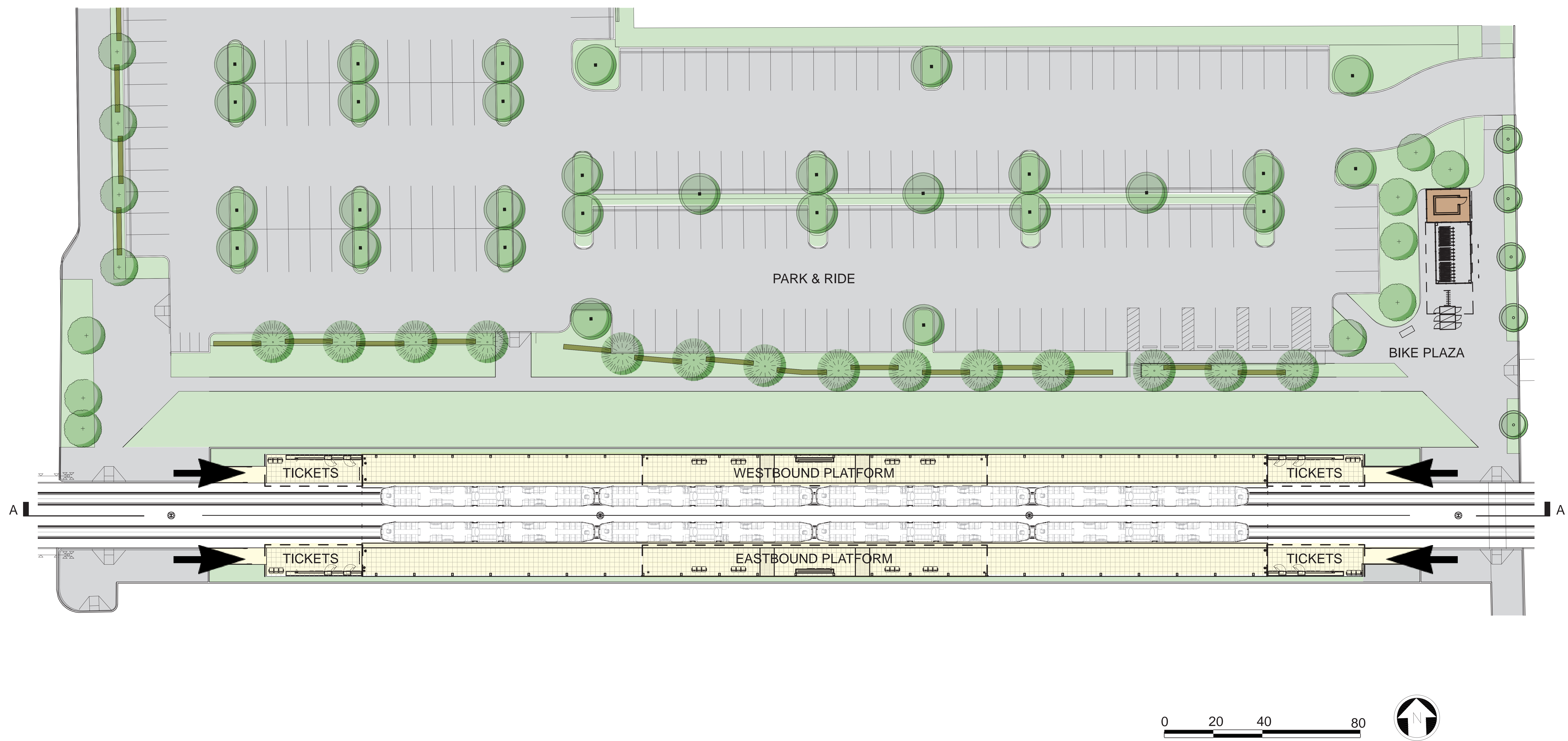
Platform plan view
