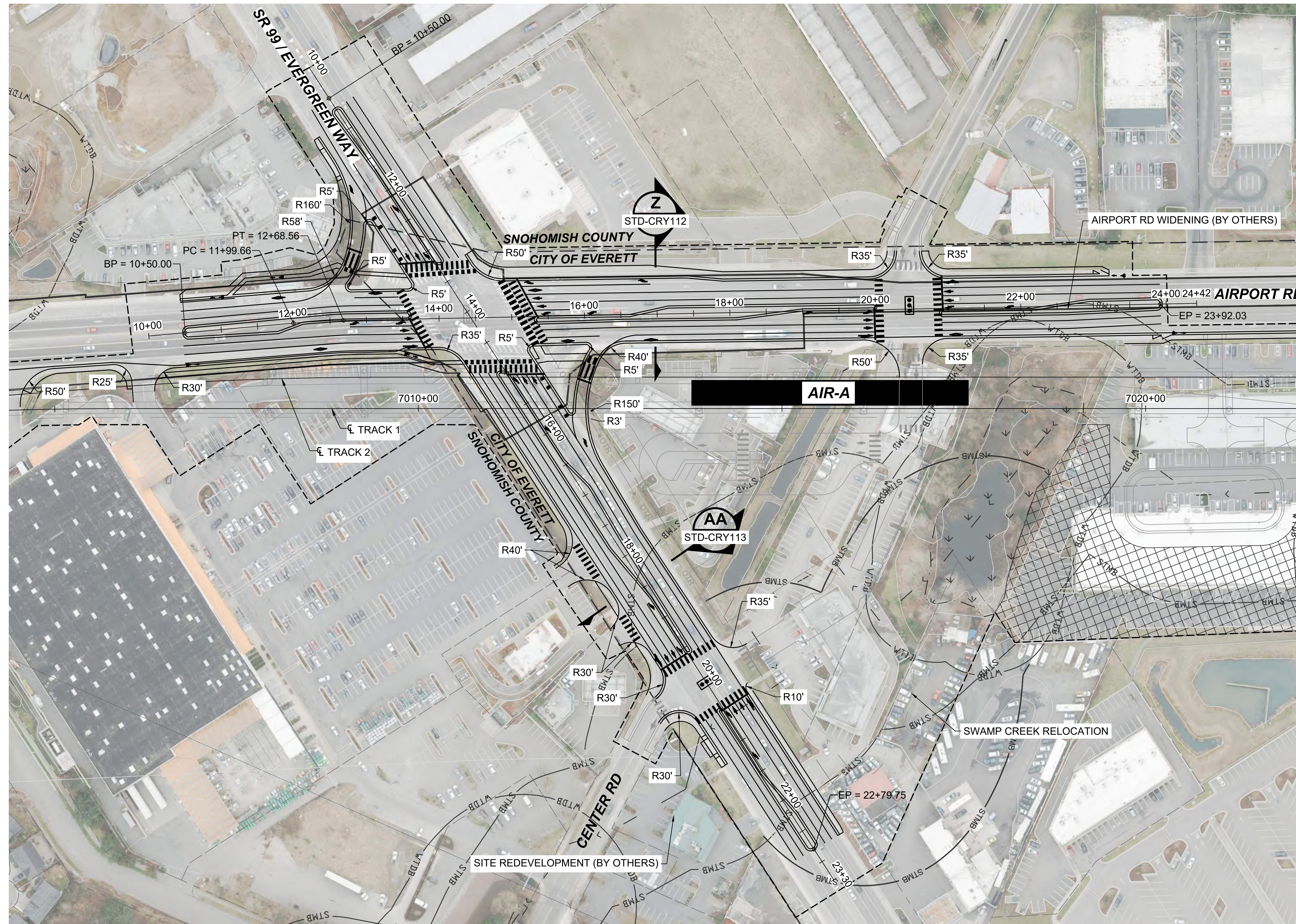
AIRPORT ROAD AND SR 99 / EVERGREEN WAY
