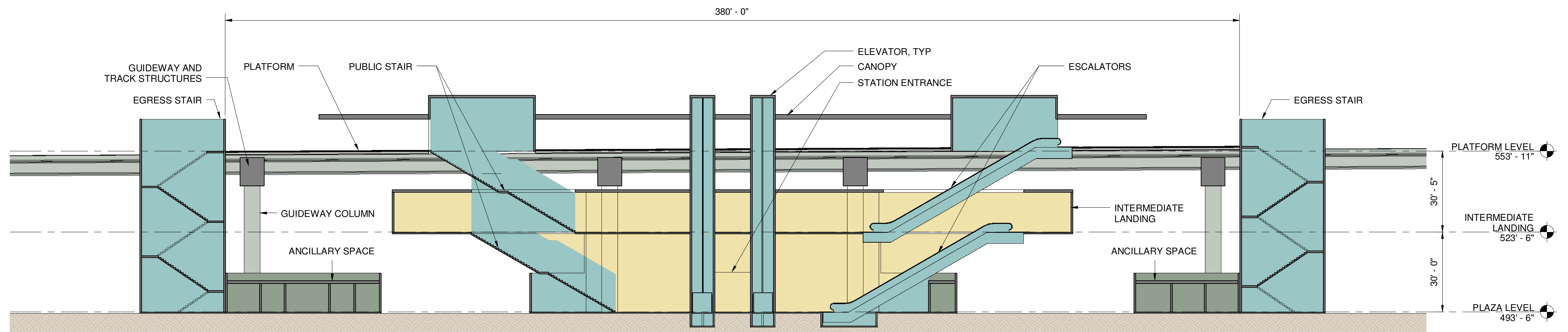
AIR-B CROSS SECTION
