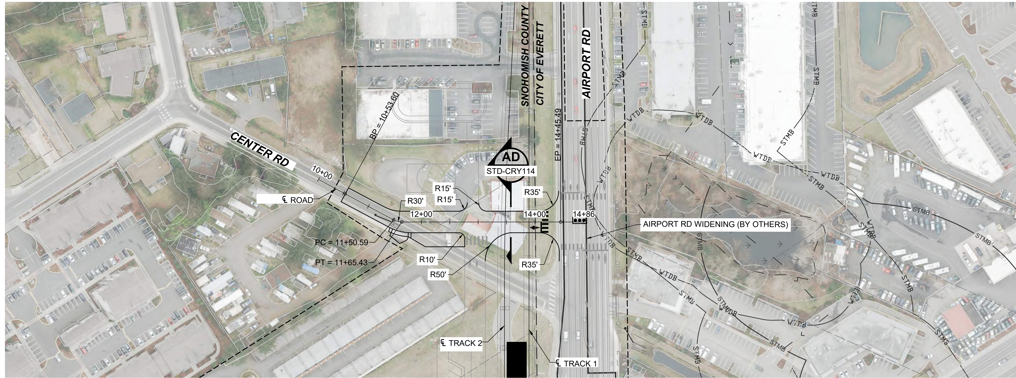
CENTER ROAD REALIGNMENT
