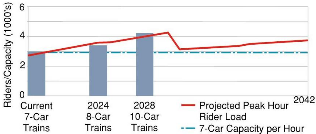
Figure ES-1 Sounder South Strategy One – Longer Trains: Peak Hour Demand Forecast and Proposed Capacities
