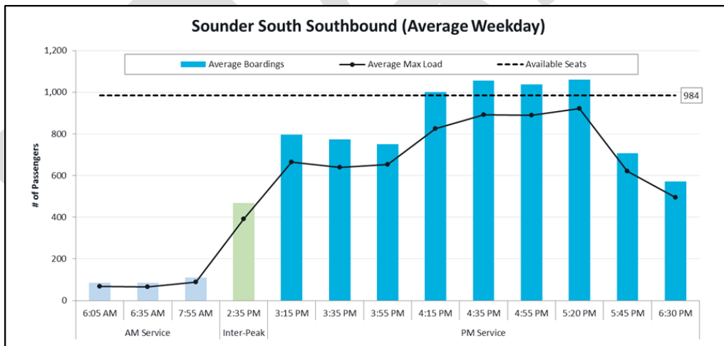
Figure 2-5 Average Weekday Boardings and Max Load (Southbound, 2018)
