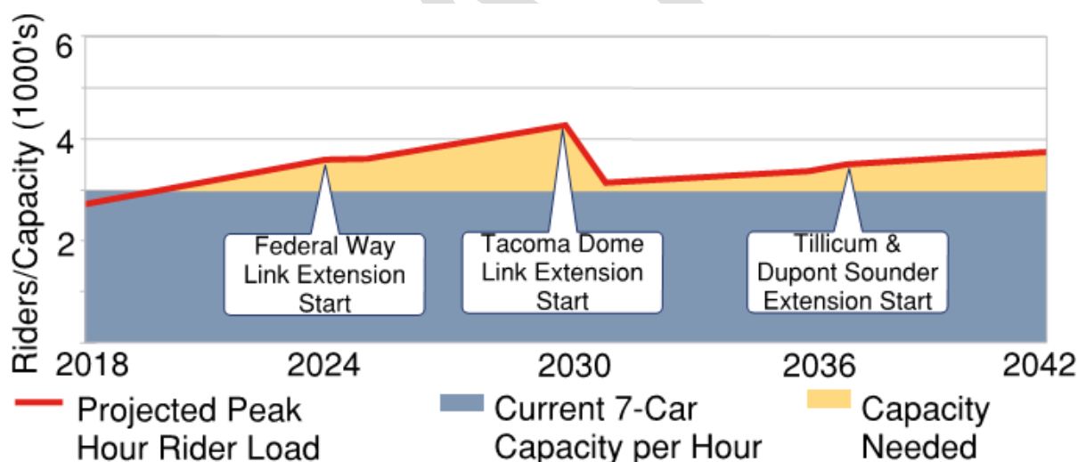
Figure ES-3 Sounder South PM Peak Hour Ridership Projections and Existing Capacity
