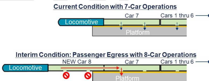
Figure 4-14 Optional Eighth Cars overhanging existing platform.
