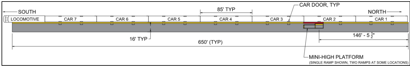
Figure 4-12 Layout of a Typical Sounder South Train and Platform Today
