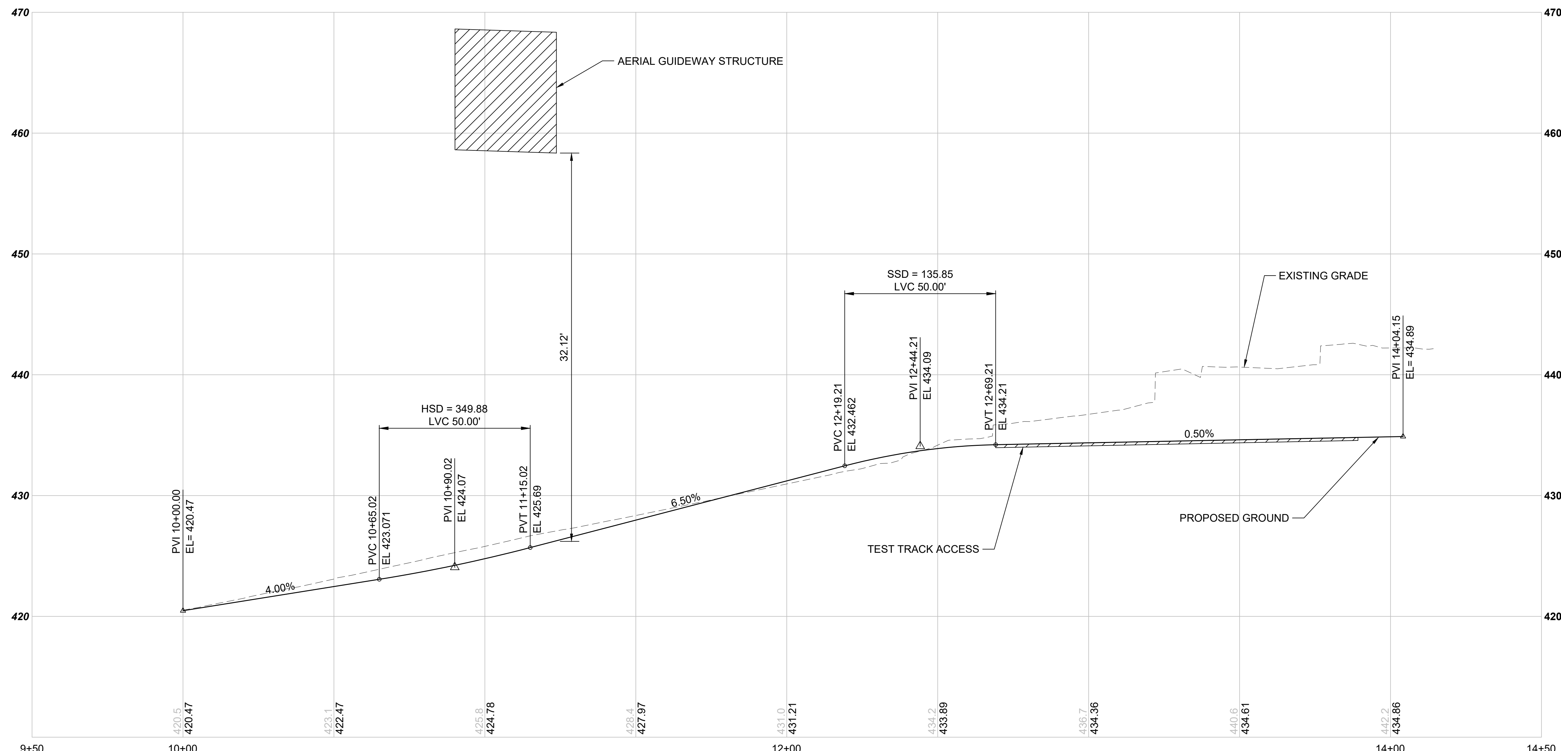
S08-R02-- TEST TRACK ACCESS ROAD STA 9+50 TO 14+50 SCALE: 1" = 20' HORIZONTAL, 1" = 5' VERTICAL
