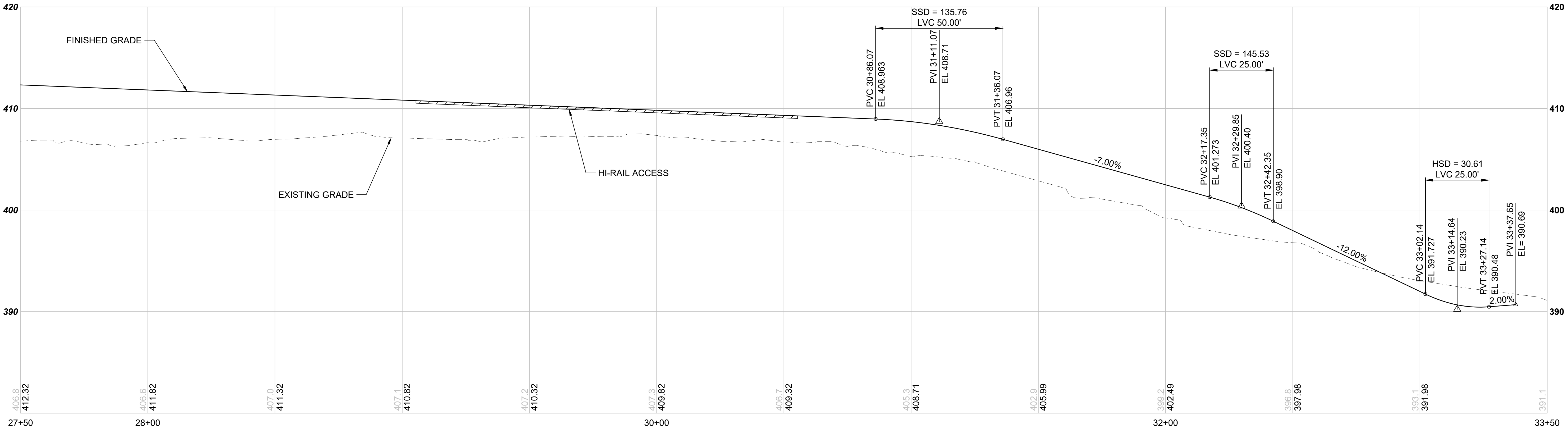
S08-R03 -- ACCESS ROAD STA 27+50 TO 33+50 SCALE: 1" = 20' HORIZONTAL, 1" = 5' VERTICAL
