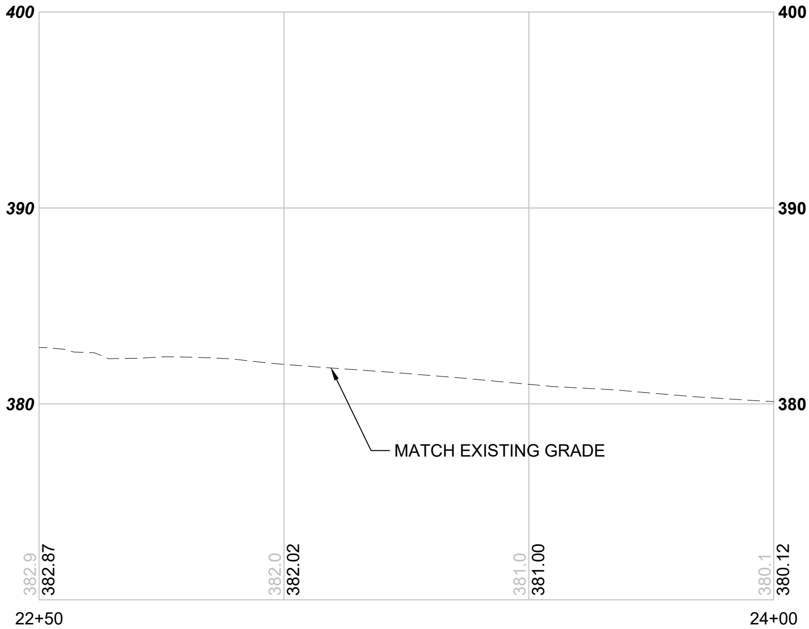
S08-R04 -- 24TH AVE S STA 22+50 TO 24+00 SCALE: 1" = 20' HORIZONTAL, 1" = 5' VERTICAL
