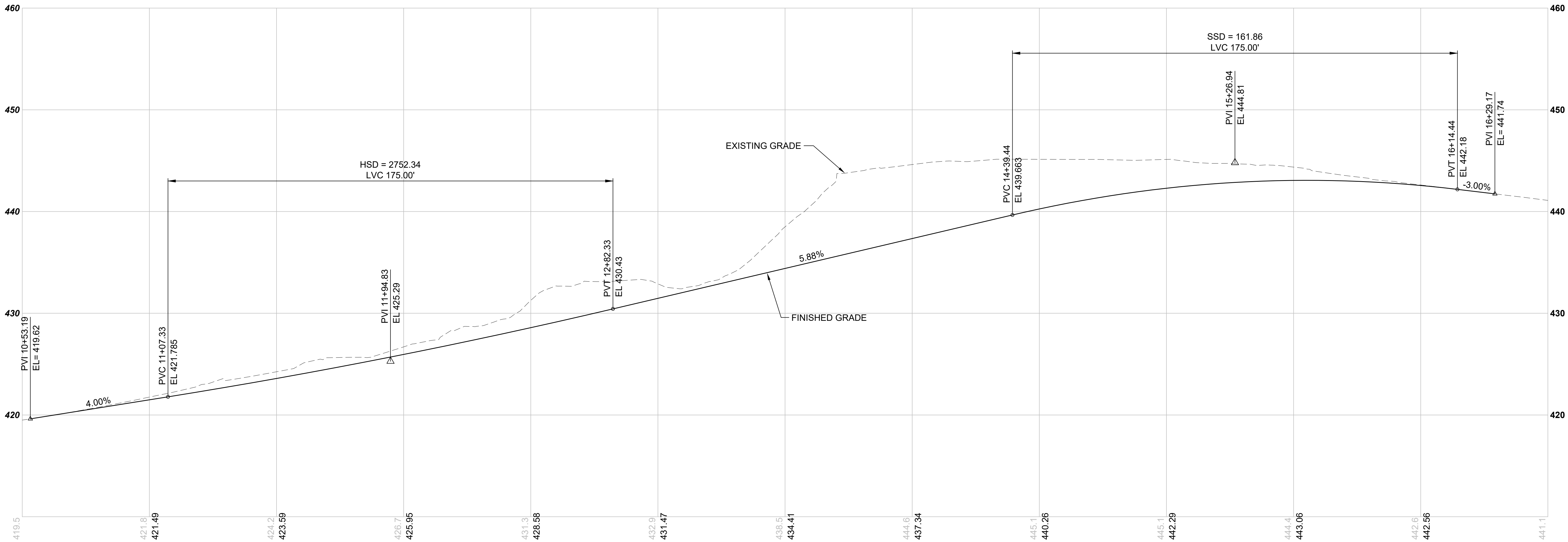
S08-R01 - WINGED FOOT WAY / OAKLAND HILLS BLVD STA 11+25 TO STA 17+25 SCALE: 1" = 20' HORIZONTAL, 1" = 5' VERTICAL
