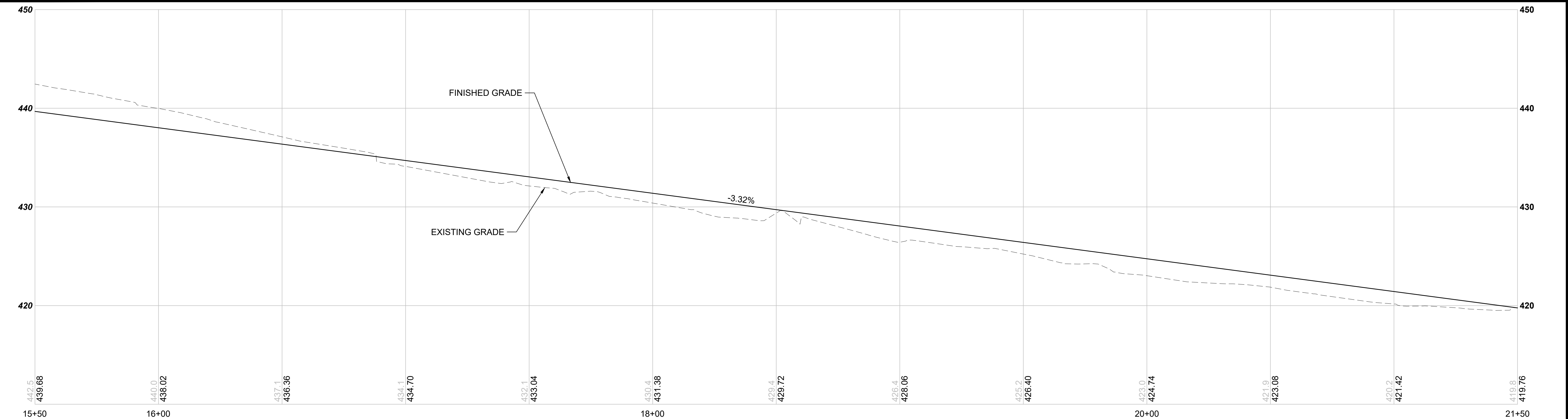
S08-R03 -- ACCESS ROAD STA 15+50 TO 21+50 SCALE: 1" = 20' HORIZONTAL, 1" = 5' VERTICAL
