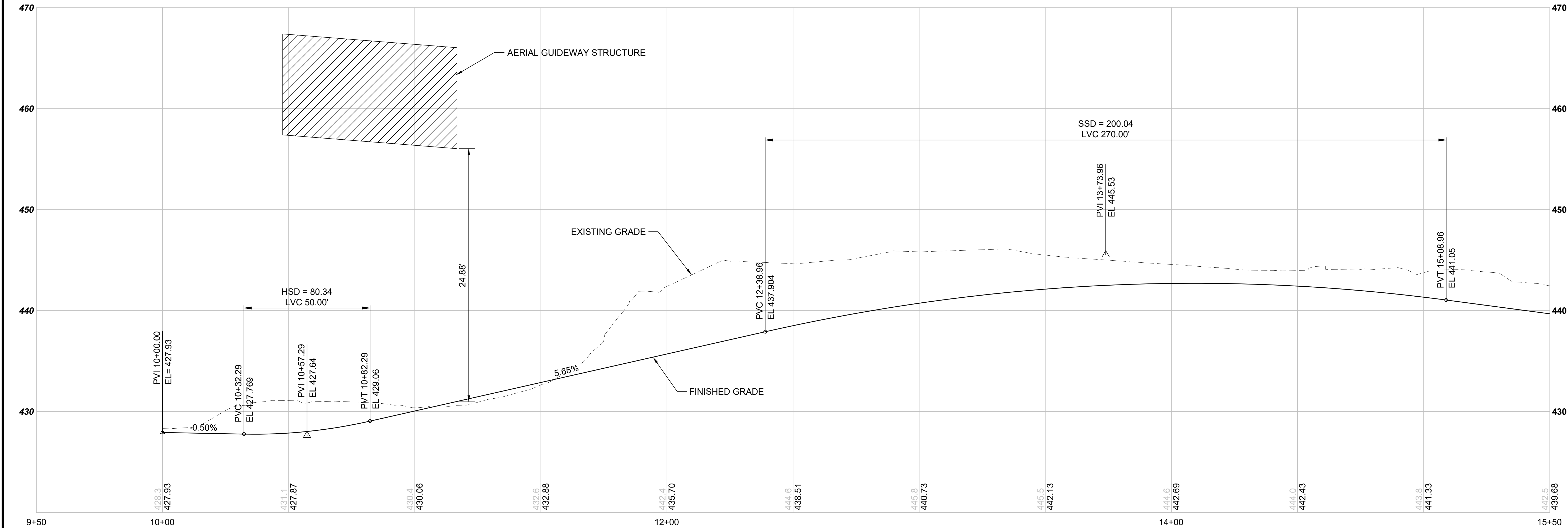
S08-R03 -- ACCESS ROAD STA 9+50 TO 15+50 SCALE: 1" = 20' HORIZONTAL, 1" = 5' VERTICAL
