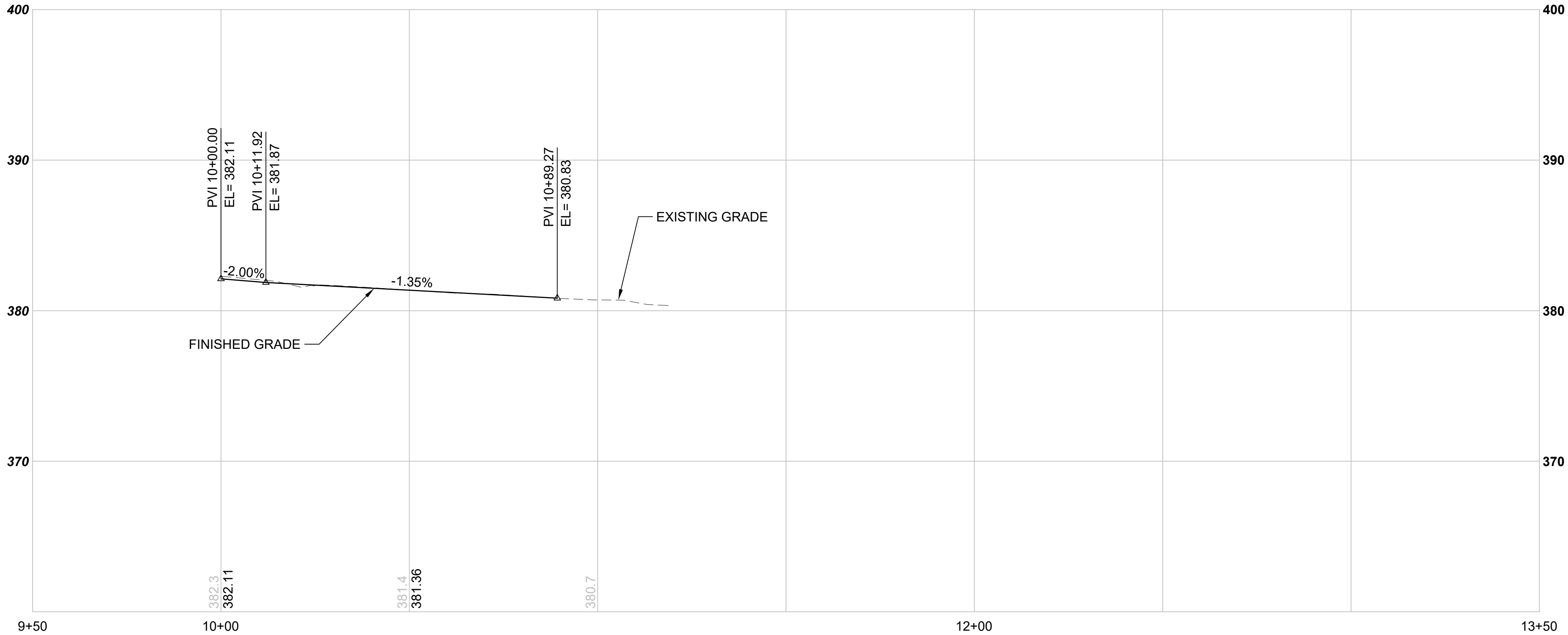
S08-R05 -- PRIVATE RESIDENTIAL DRIVEWAY STA 9+50 TO 13+50 SCALE: 1" = 20' HORIZONTAL, 1" = 5' VERTICAL
