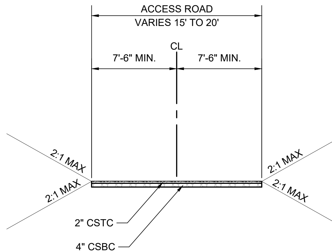
POND ACCESS ROAD FEDERAL WAY
