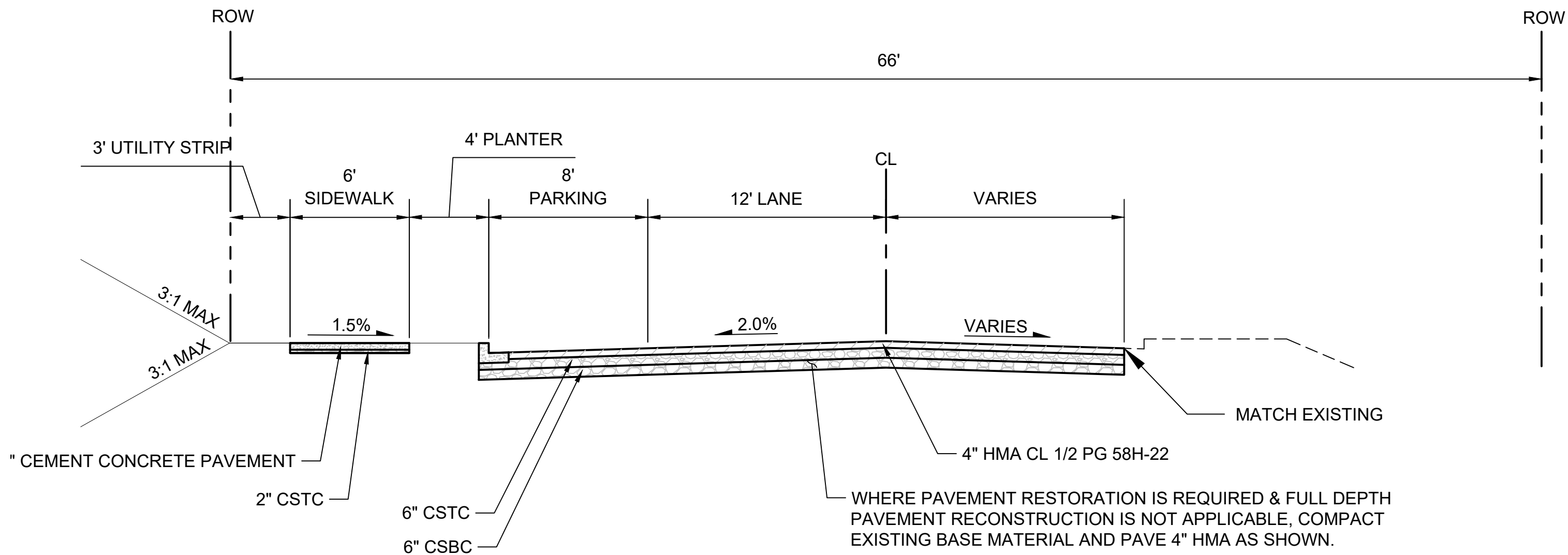
S 344TH ST IMPROVEMENTS FEDERAL WAY TYPICAL SECTION 3-2R PER DEVELOPMENT STANDARDS
