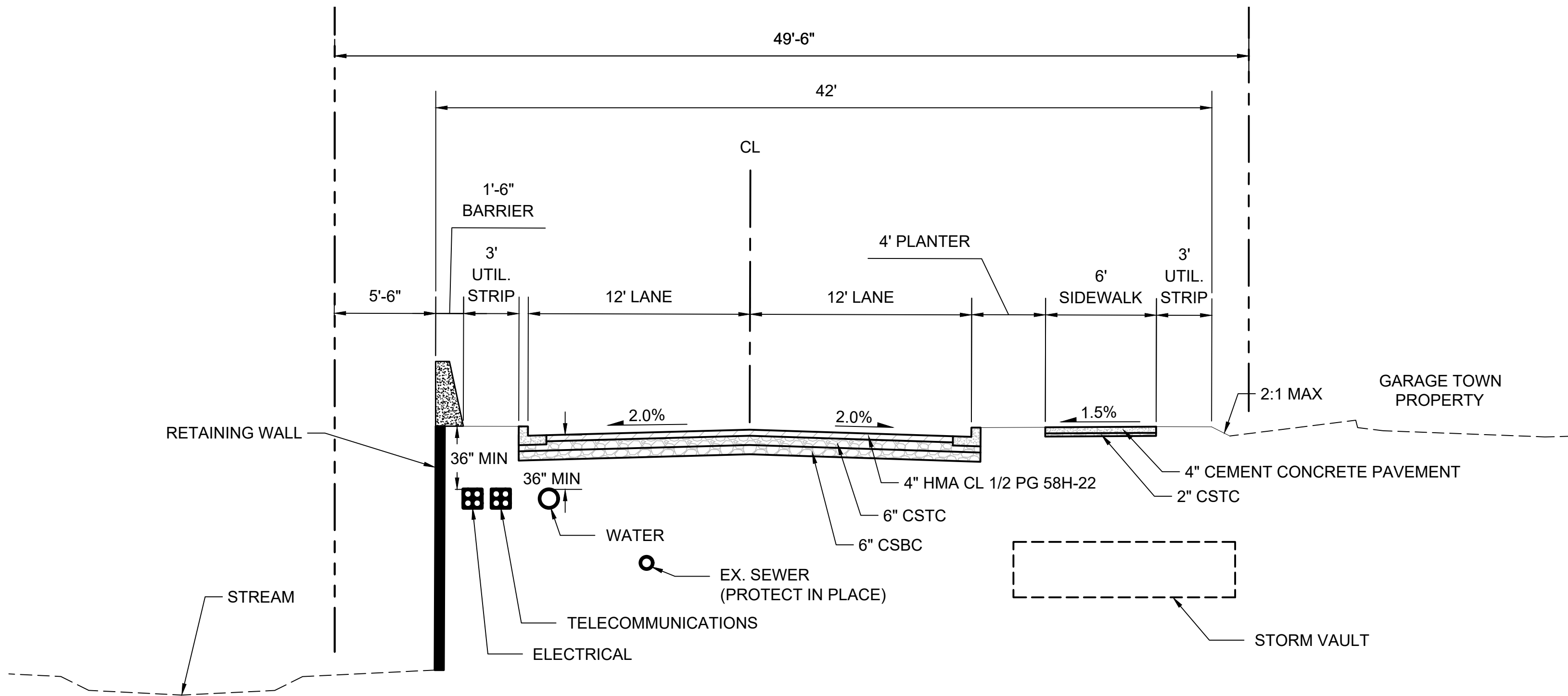
S 21ST AVE EXTENSION FEDERAL WAY
