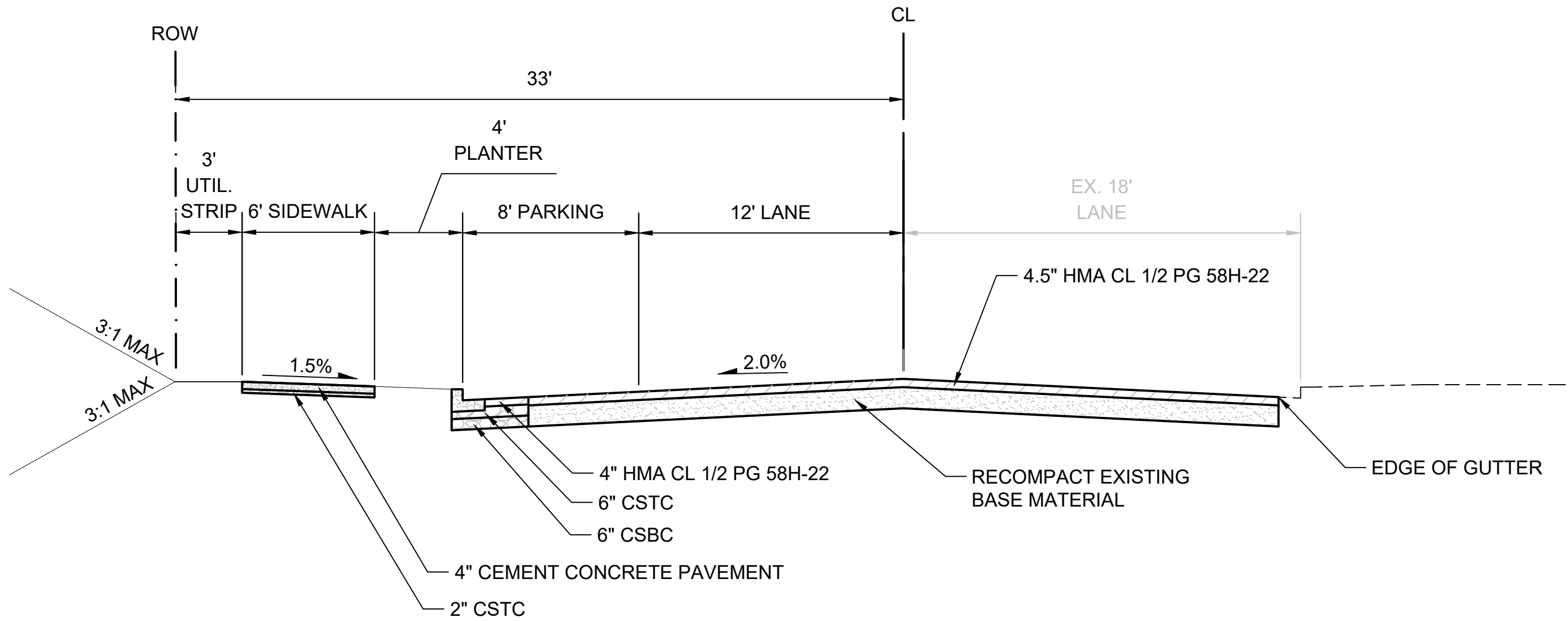
S 341ST PL HALF-STREET FRONTAGE IMPROVEMENTS FEDERAL WAY TYPICAL SECTION 3-2R PER DEVELOPMENT STANDARDS
