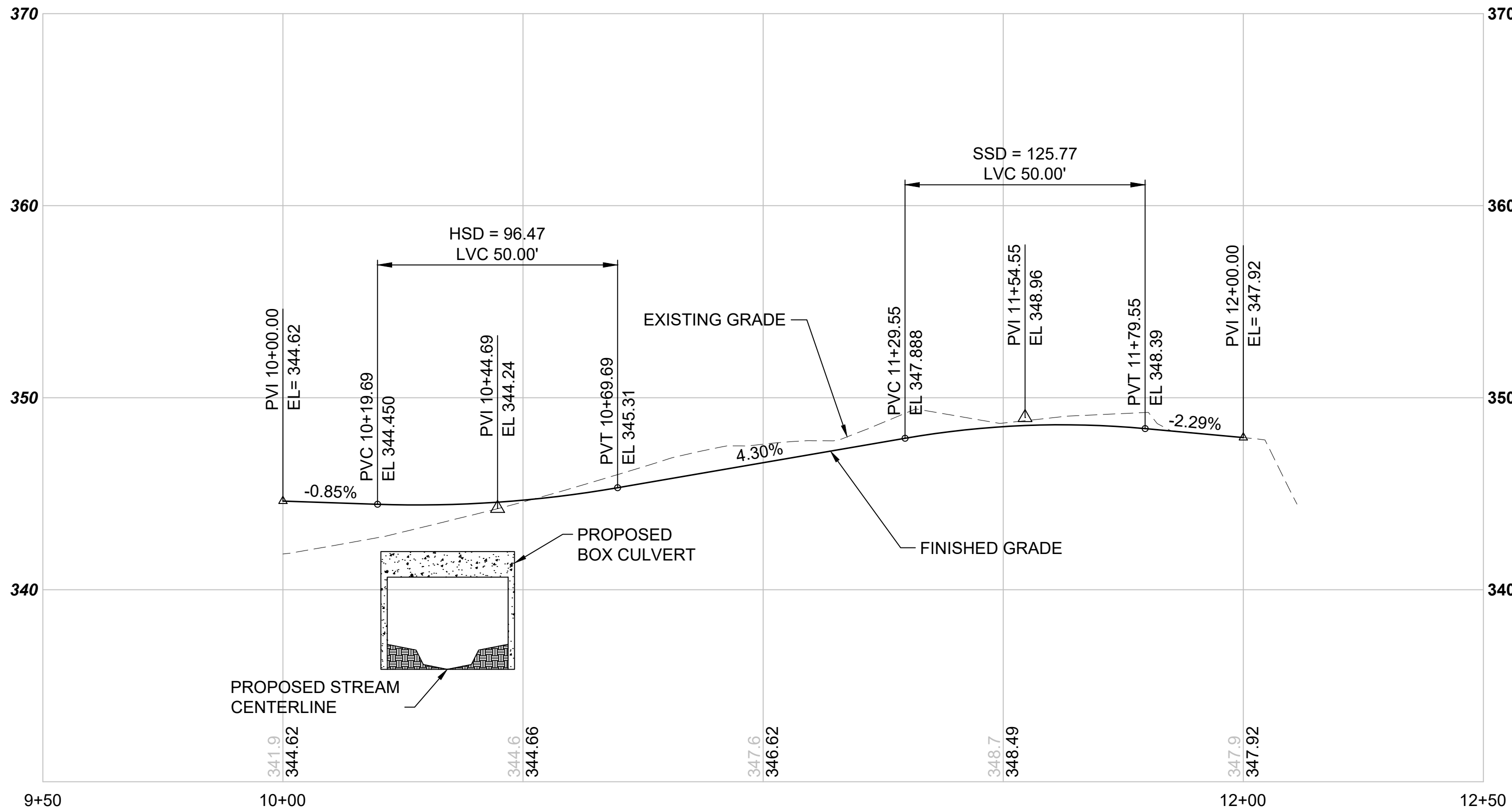
M08-R09 -- WSDOT POND ACCESS ROAD STA 9+50 TO 12+50 SCALE: 1" = 20' HORIZONTAL, 1" = 5' VERTICAL
