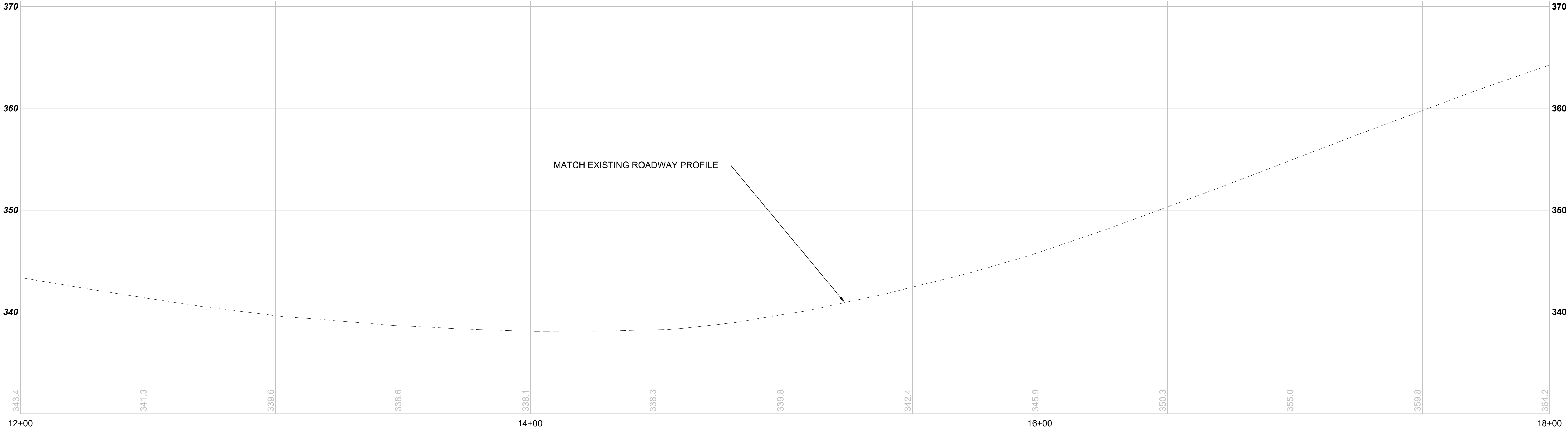
M08-R01 -- S 336TH ST STA 12+00 TO 18+00 SCALE: 1" = 20' HORIZONTAL, 1" = 5' VERTICAL
