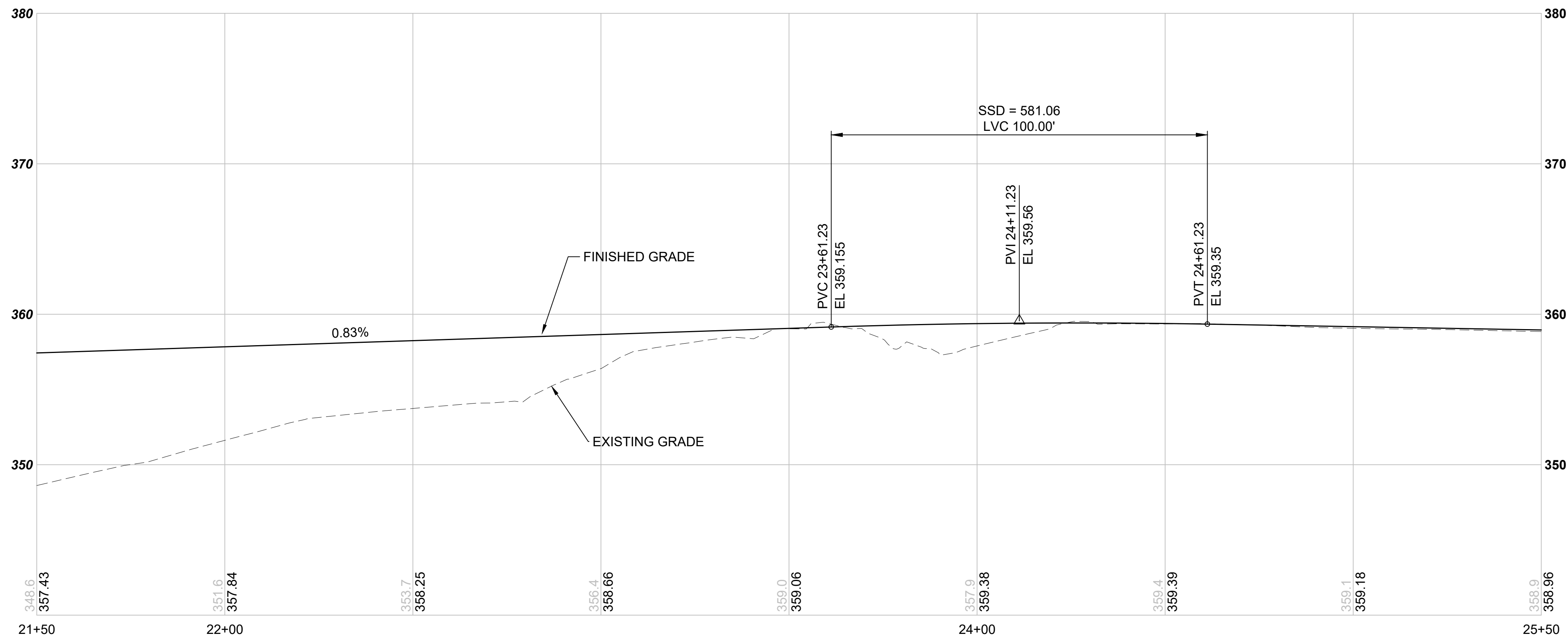
M08-R02 -- 18TH PL S EXTENSION STA 21+50 TO 25+50 SCALE: 1" = 20' HORIZONTAL, 1" = 5' VERTICAL
