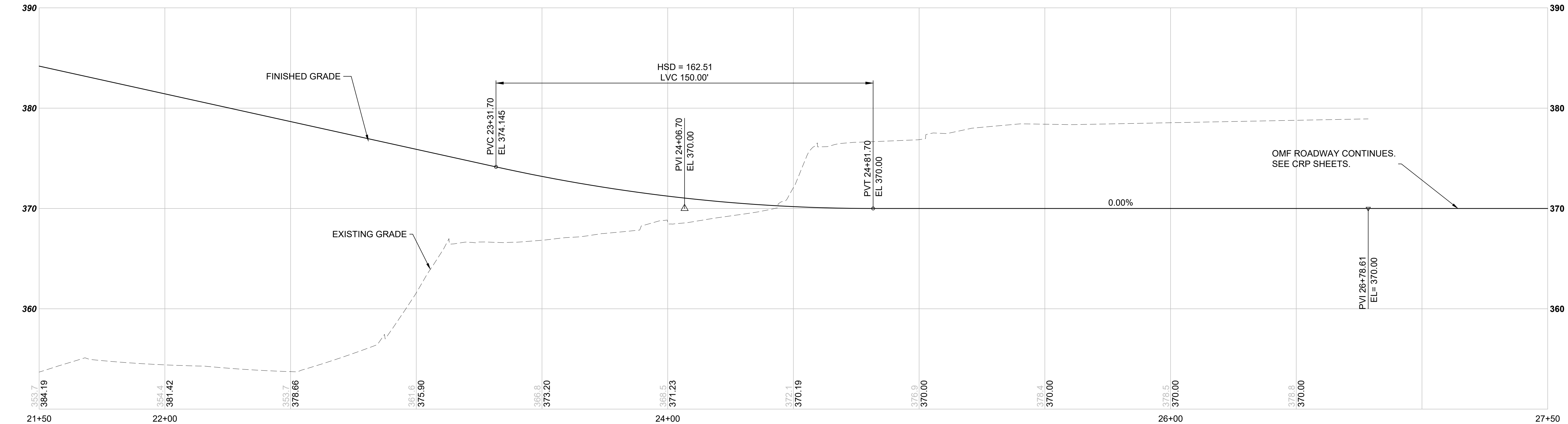
M08-R04 -- GUARD GATE ENTRANCE & OMF ACCESS ROAD STA 21+50 TO 27+50 SCALE: 1" = 20' HORIZONTAL, 1" = 5' VERTICAL
