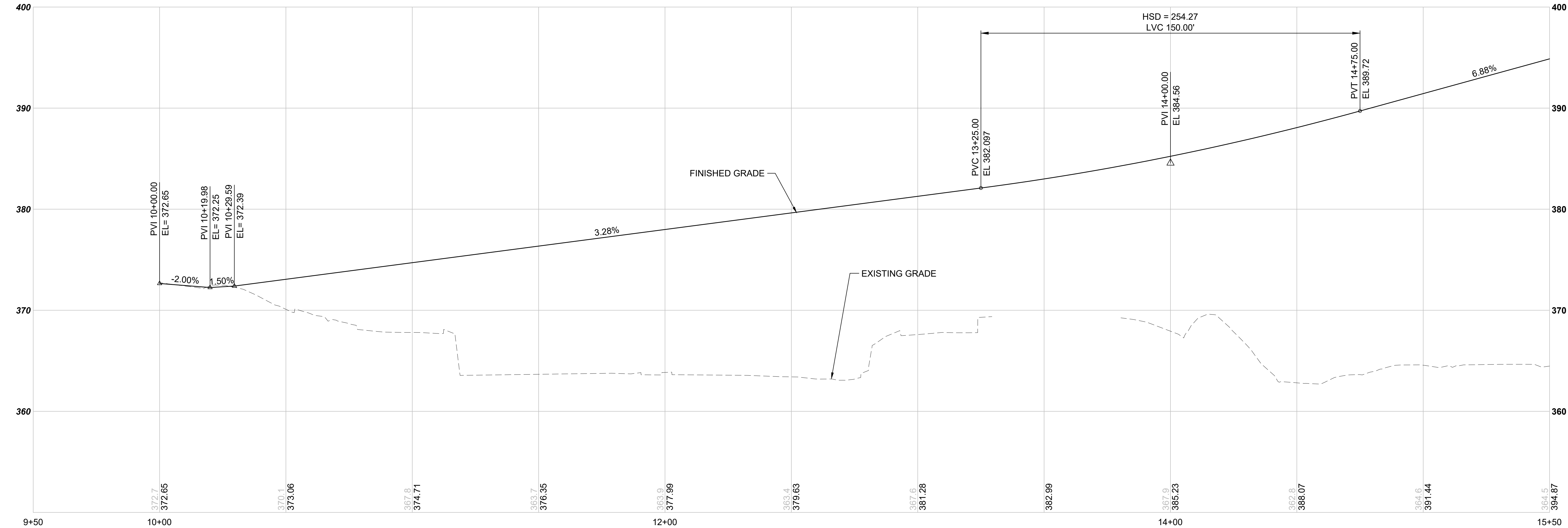
M08-R04 -- GUARD GATE ENTRANCE & OMF ACCESS ROAD STA 9+50 TO 15+50 SCALE: 1" = 20' HORIZONTAL, 1" = 5' VERTICAL
