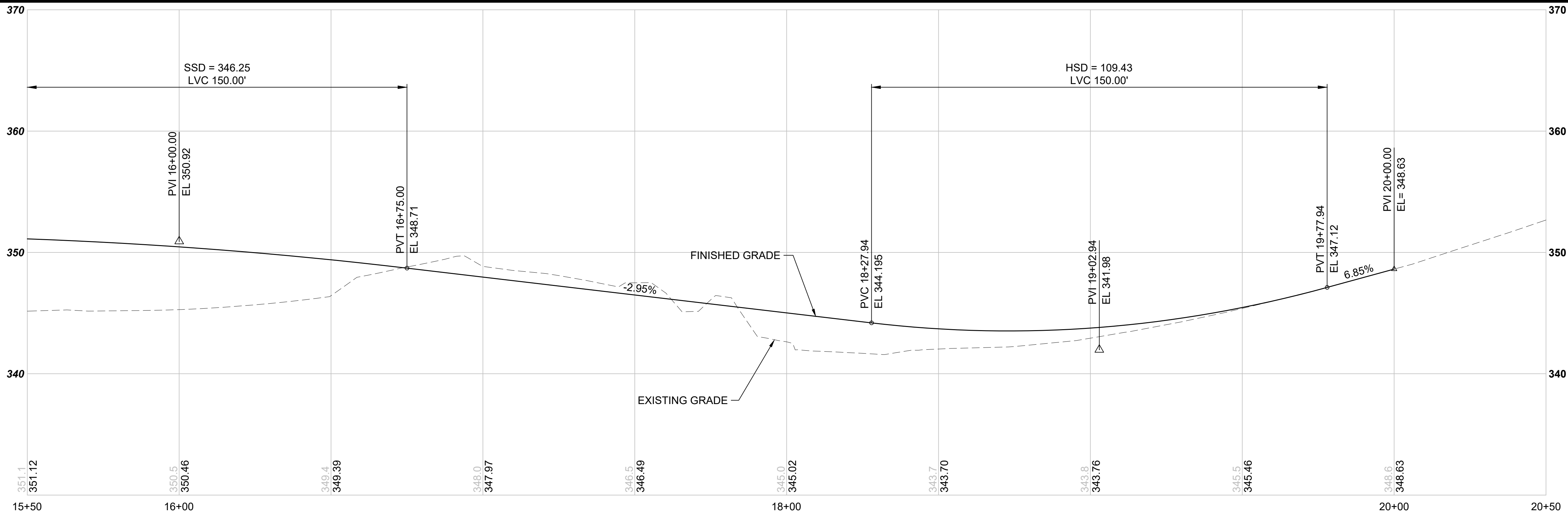
M08-R08 -- 21ST AVE S EXTENSION STA 15+50 TO 20+50 SCALE: 1" = 20' HORIZONTAL, 1" = 5' VERTICAL
