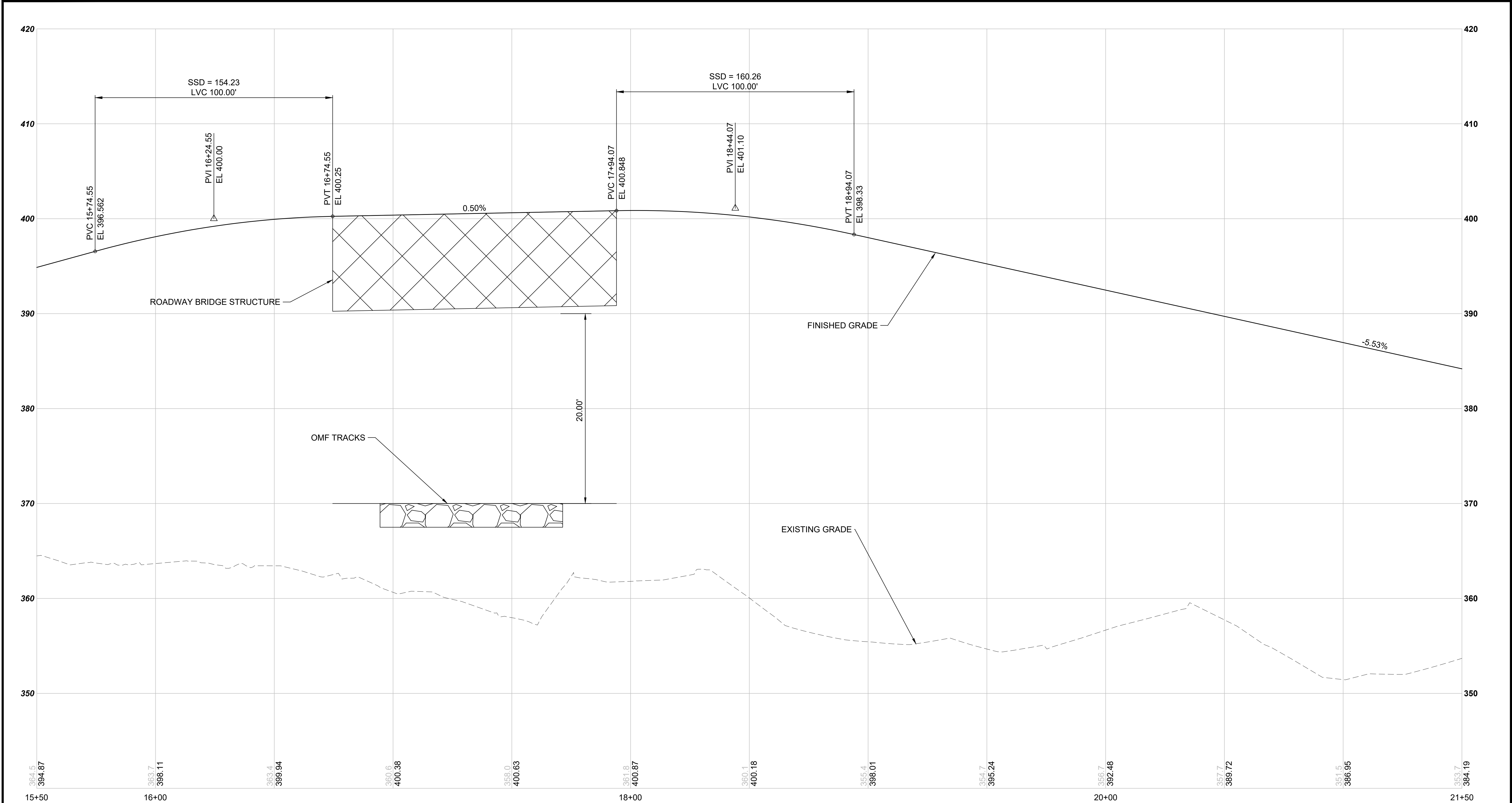
M08-R04 -- GUARD GATE ENTRANCE & OMF ACCESS ROAD STA 15+50 TO 21+50 SCALE: 1" = 20' HORIZONTAL, 1" = 5' VERTICAL
