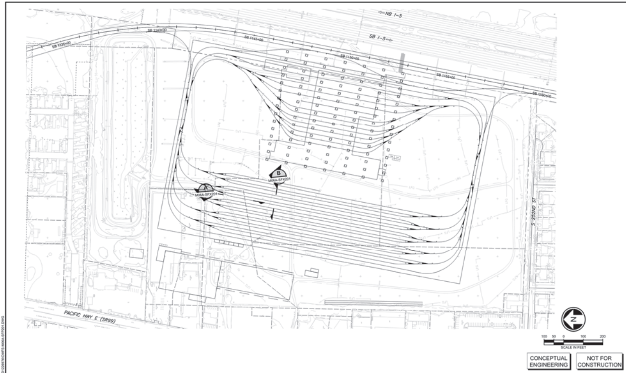
Figure 2-5. Hybrid 2 Shaft Layout
