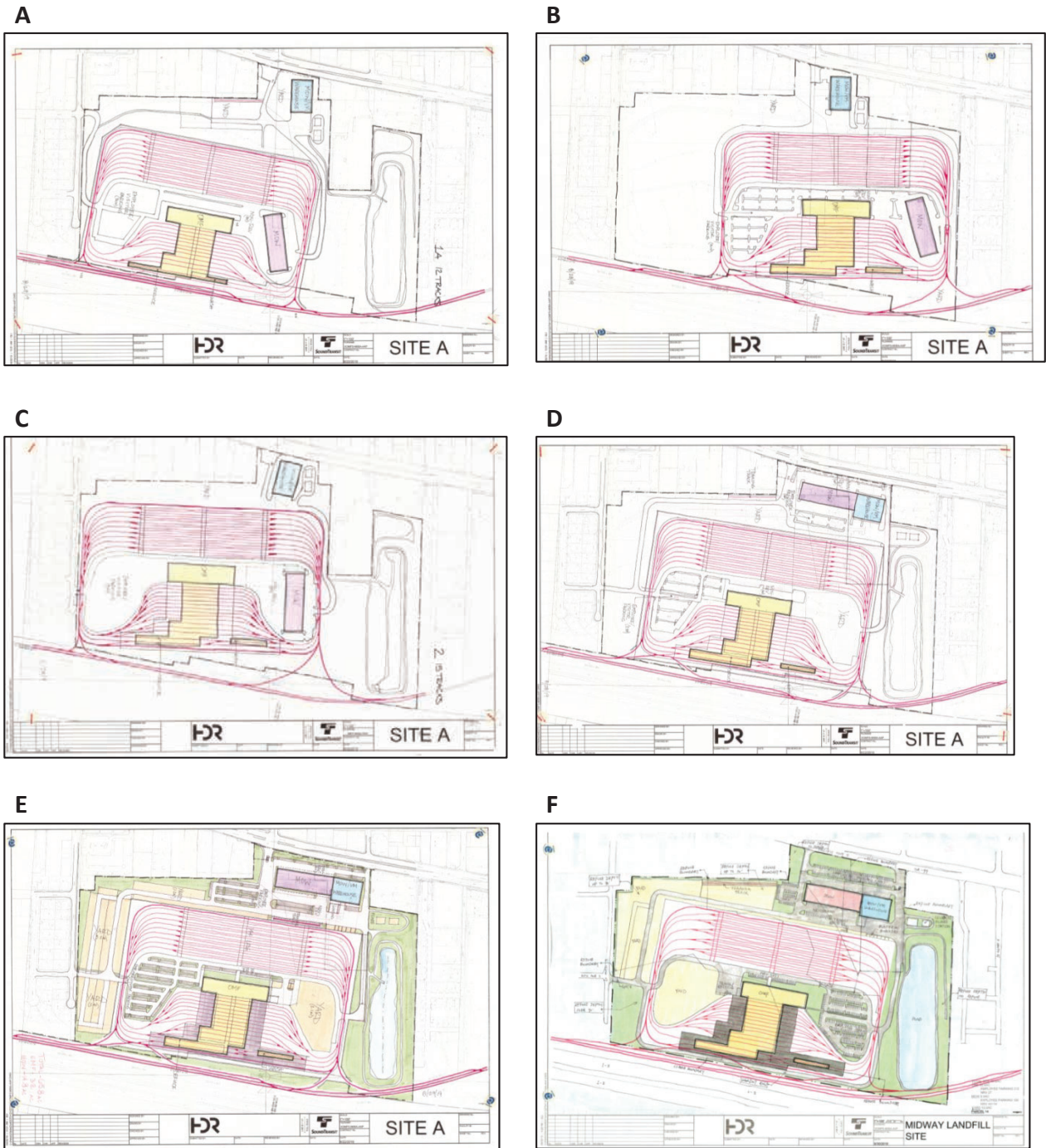
EXHIBIT 4-1 Evolution/Optimization of Midway Site Layouts
