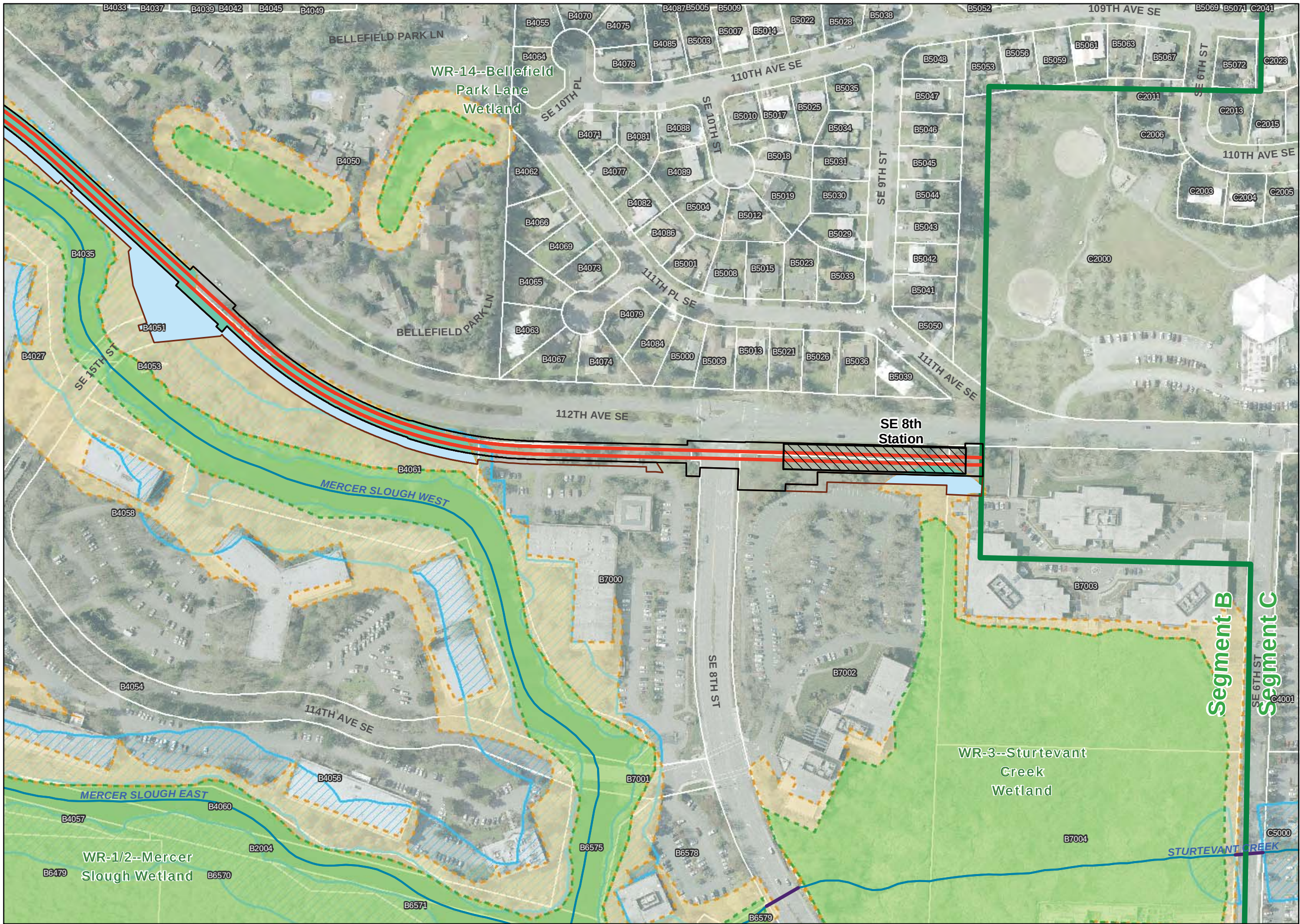
Exhibit F-10 Wetland, Wetland Buffer, and Wetland Mitigation Impacts Alternative B2M to C9T Sheet 5 East Link Project
