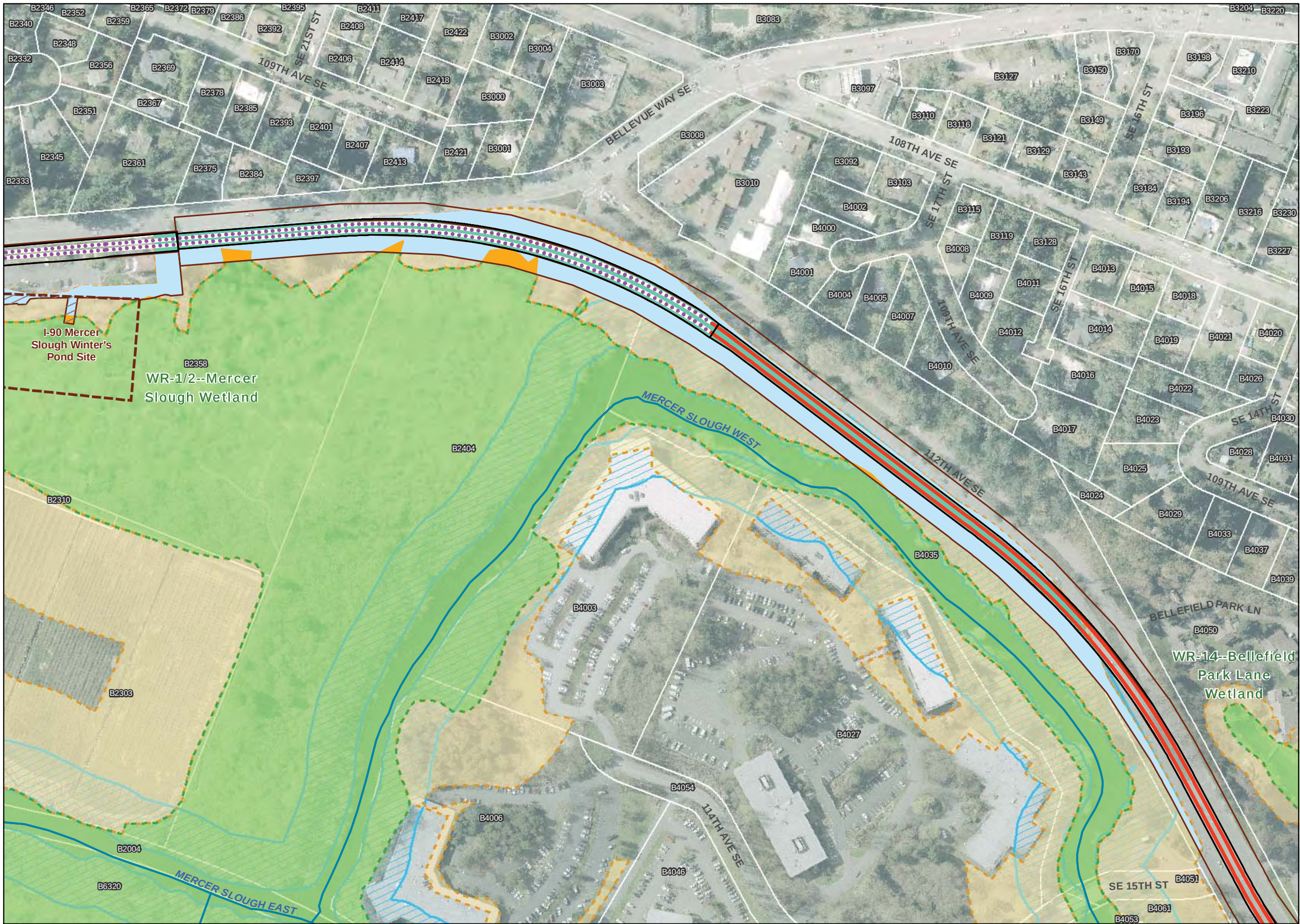
Exhibit F-4 Wetland, Wetland Buffer, and Wetland Mitigation Impacts Alternative B2M to C11A Sheet 4 East Link Project
