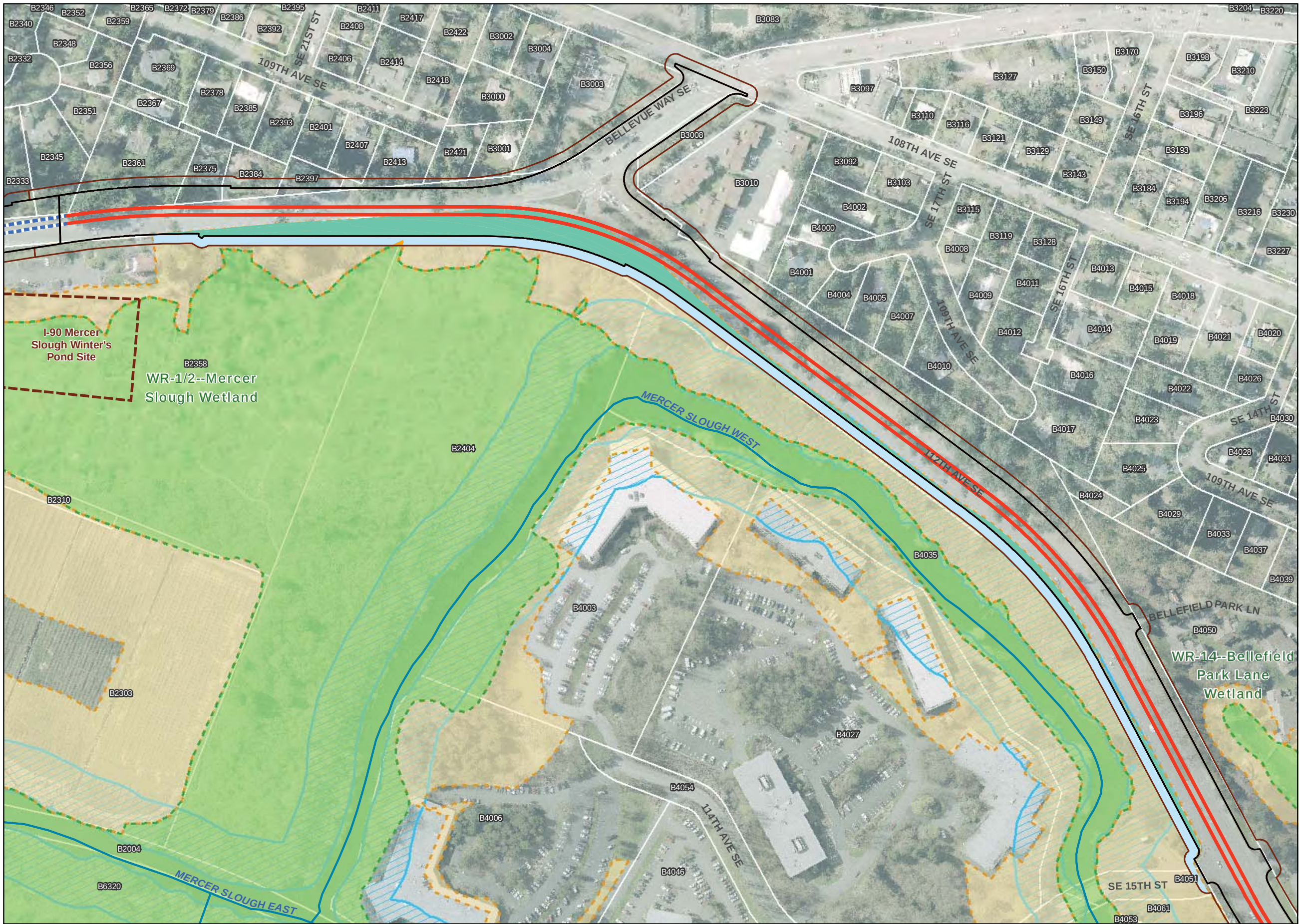
Exhibit F-19 Wetland, Wetland Buffer, and Wetland Mitigation Impacts Alternative B2A Sheet 4 East Link Project
