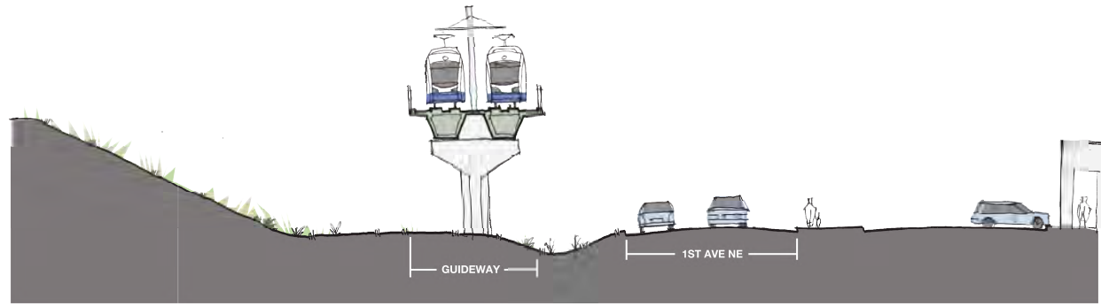
SECTION 4 LOOKING NORTH ELEVATED GUIDEWAY AT NE 98TH ST
