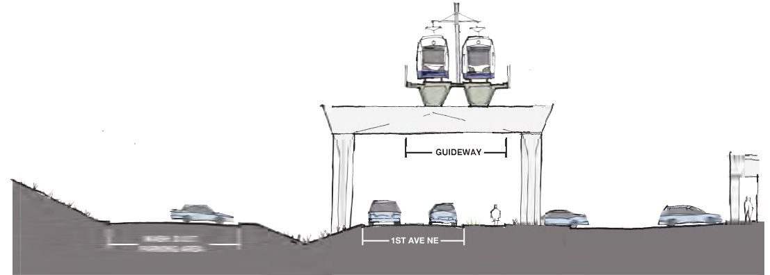
SECTION 5 LOOKING NORTH ELEVATED GUIDEWAY AT NE 100TH ST
