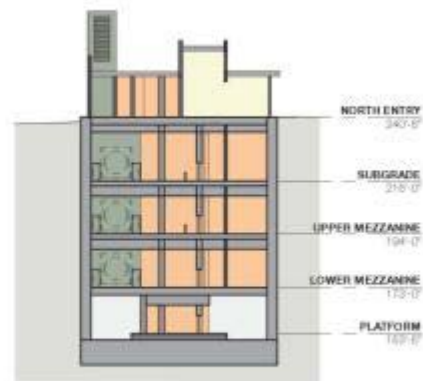
Cross Section - S2
