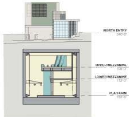
Cross Section - S1
