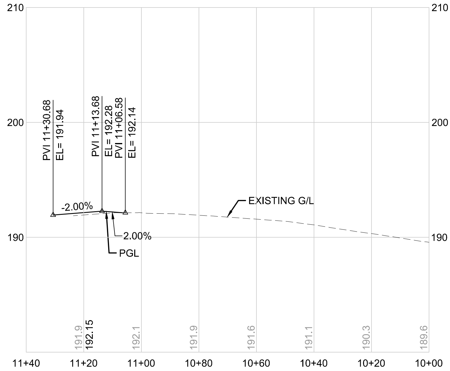
BRS243 N-S LINE HORIZONTAL SCALE: 1"=20' VERTICAL SCALE: 1"=5'
