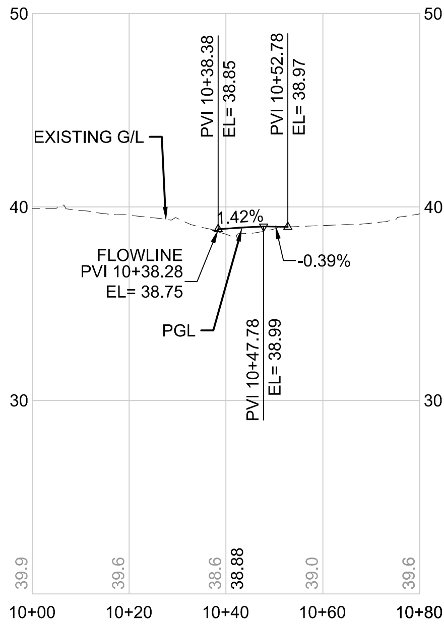
BRS337 LINE HORIZONTAL SCALE: 1"=20' VERTICAL SCALE: 1"=5'
