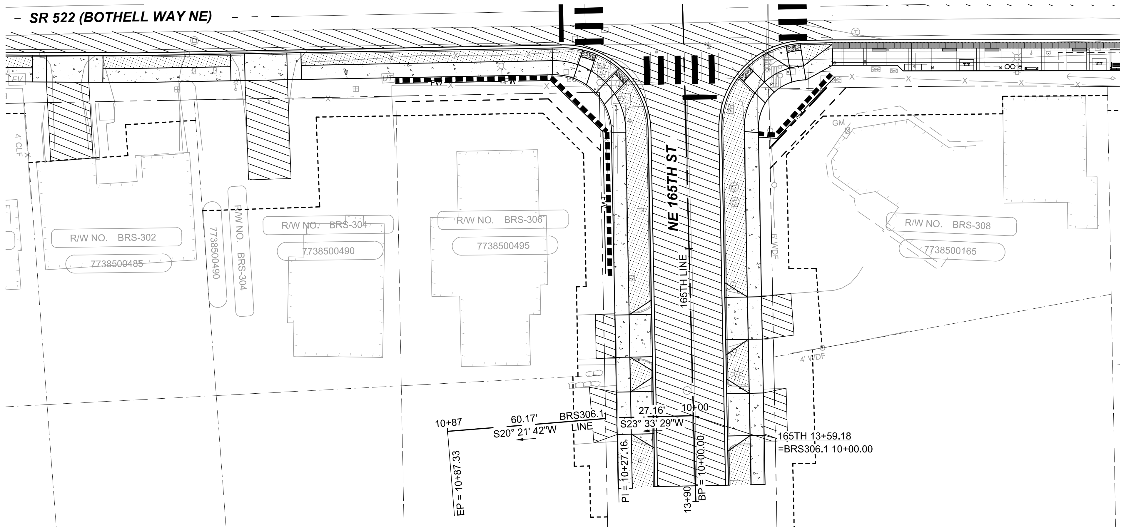
BRS306.1 LINE HORIZONTAL SCALE: 1"=20' VERTICAL SCALE: 1"=5'
