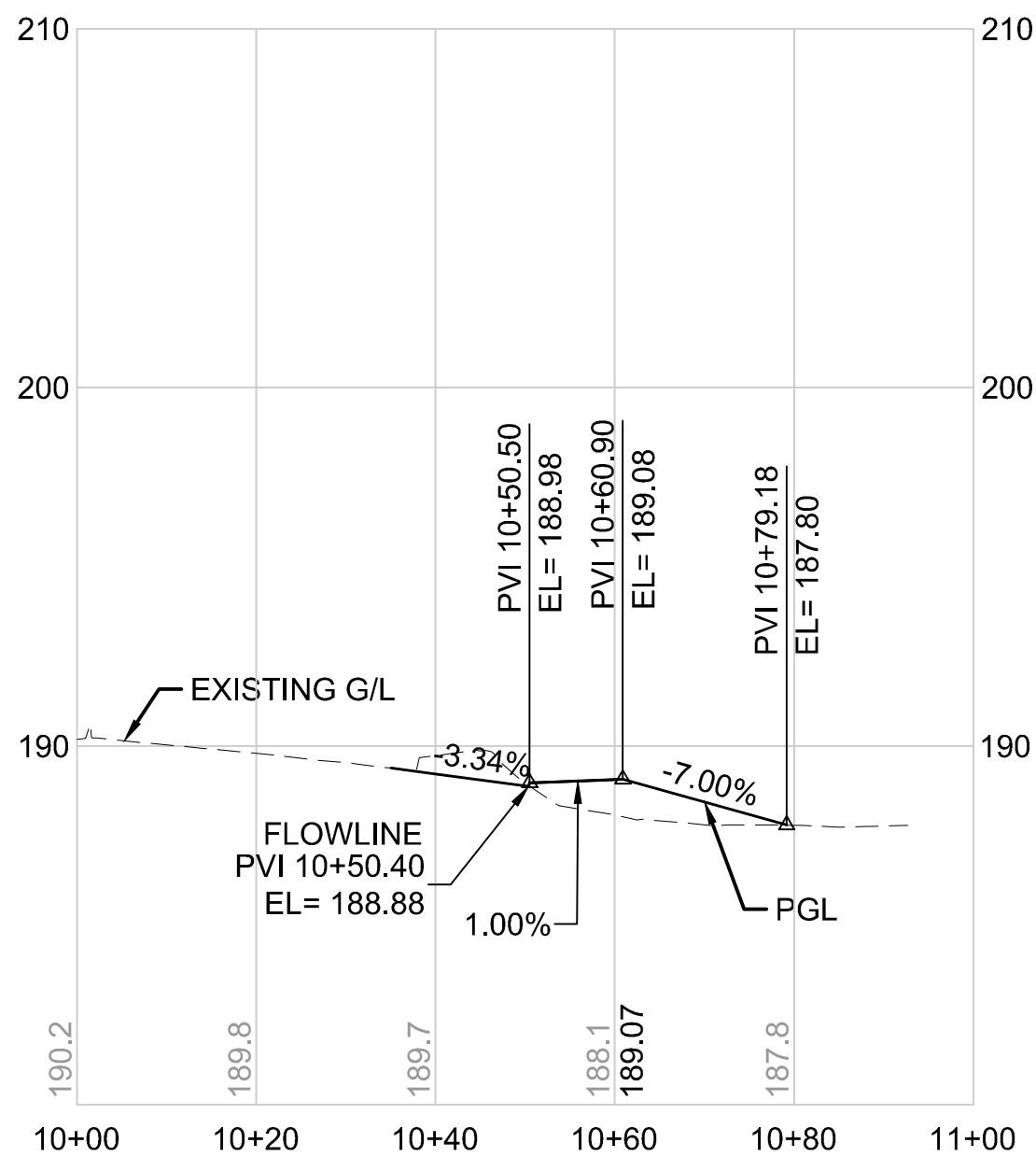
BRS246 LINE HORIZONTAL SCALE: 1"=20' VERTICAL SCALE: 1"=5'
