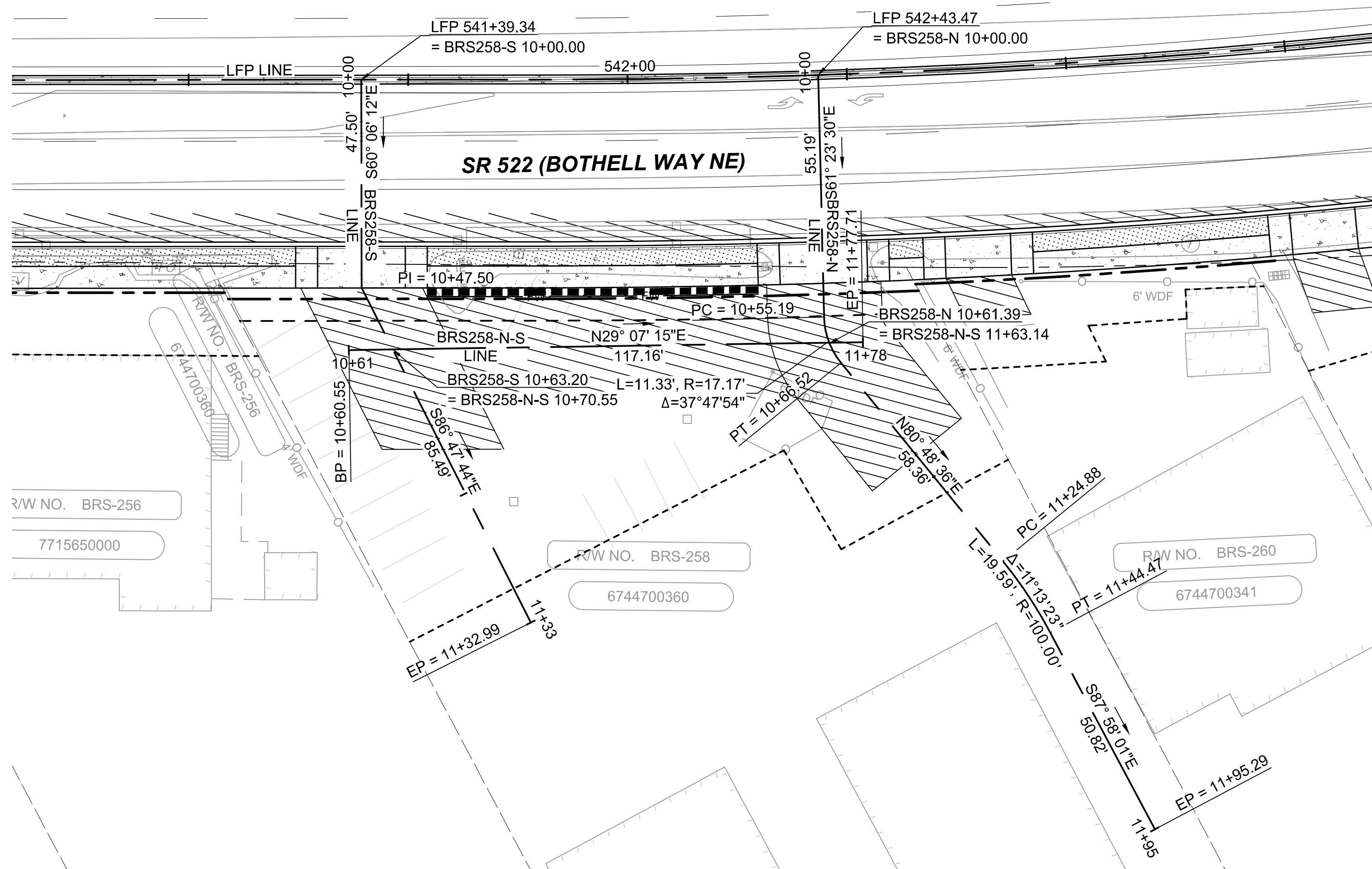
BRS258 N-S LINE HORIZONTAL SCALE: 1"=20' VERTICAL SCALE: 1"=5'
