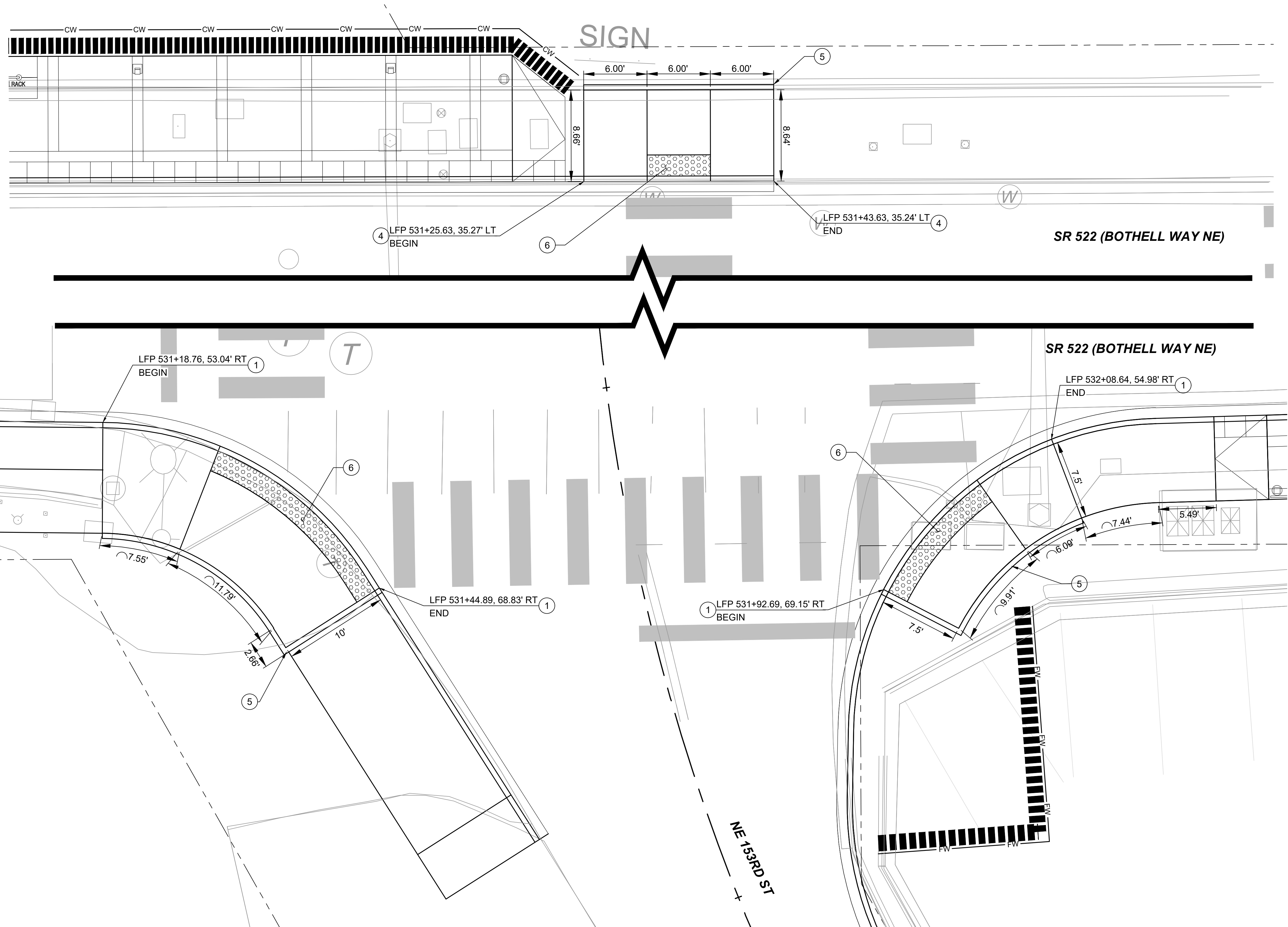
CURB RAMP DETAIL SCALE: 1" = 5'
