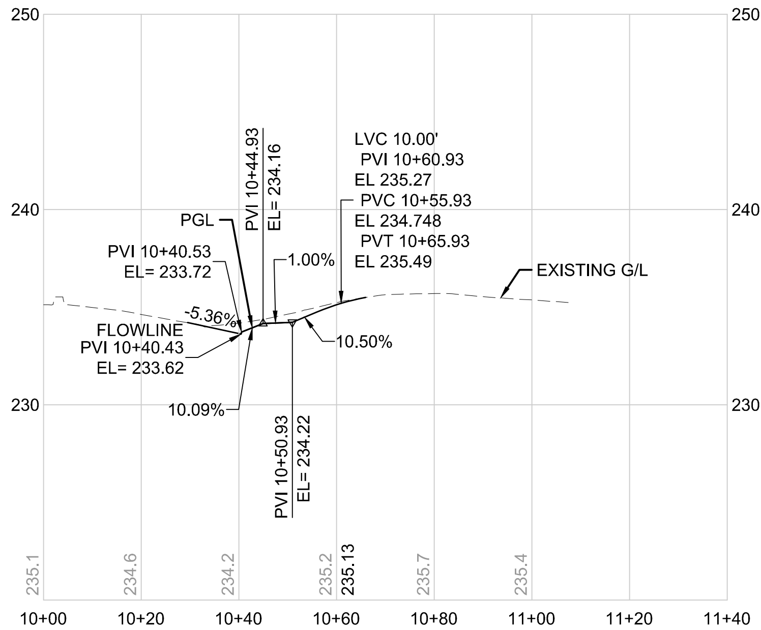
BRS223 LINE HORIZONTAL SCALE: 1"=20' VERTICAL SCALE: 1"=5'
