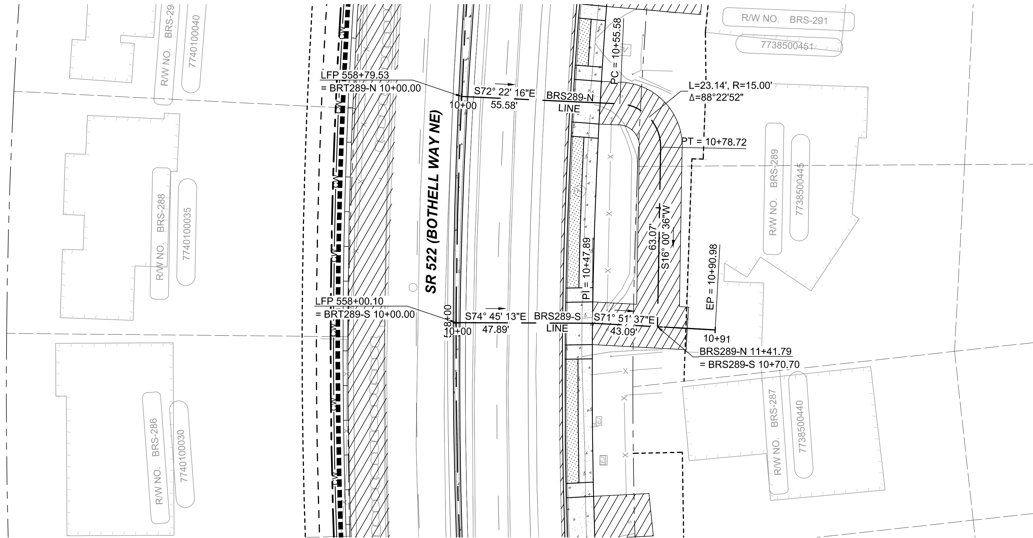
BRS289-S LINE HORIZONTAL SCALE: 1"=20' VERTICAL SCALE: 1"=5'
