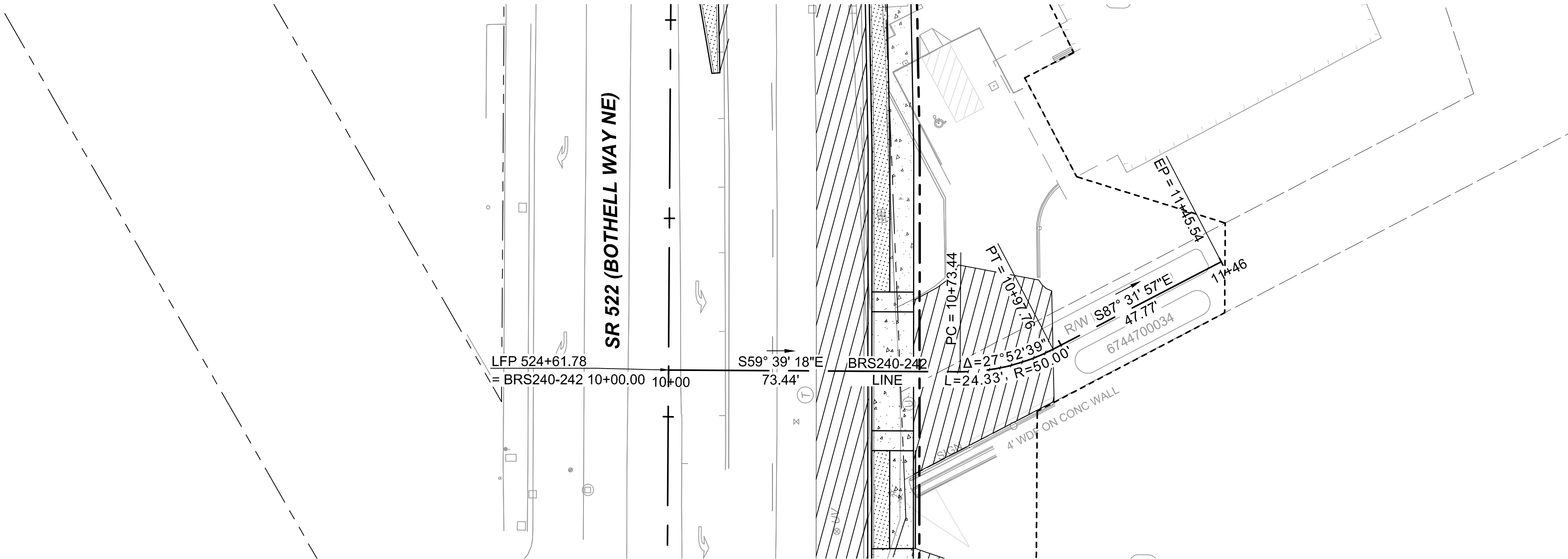
BRS240-242 LINE HORIZONTAL SCALE: 1"=20' VERTICAL SCALE: 1"=5'
