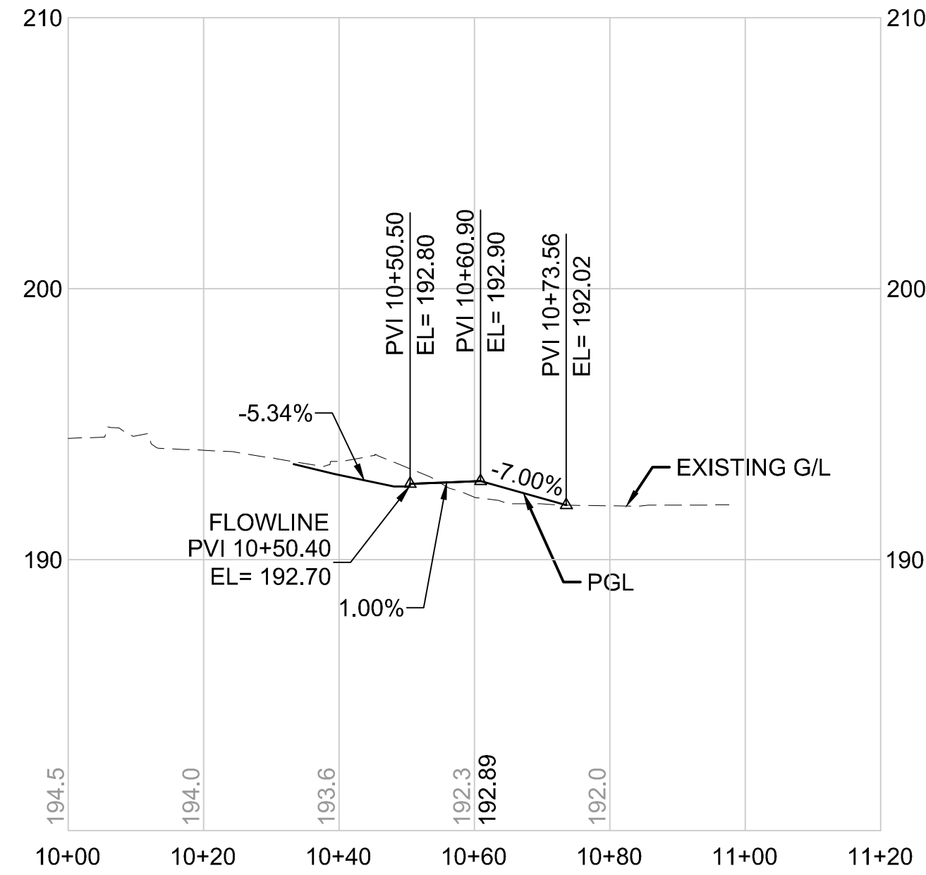
BRS243-S LINE HORIZONTAL SCALE: 1"=20' VERTICAL SCALE: 1"=5'
