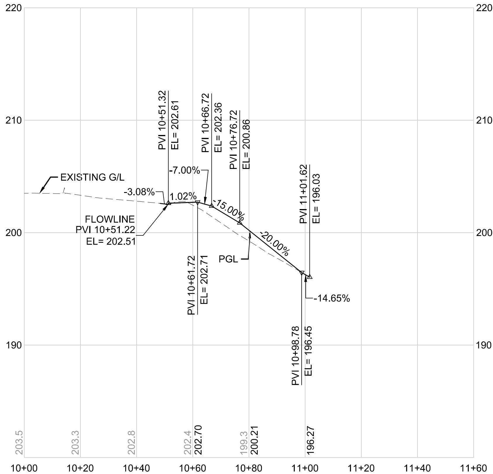
BRS240-242 LINE HORIZONTAL SCALE: 1"=20' VERTICAL SCALE: 1"=5'
