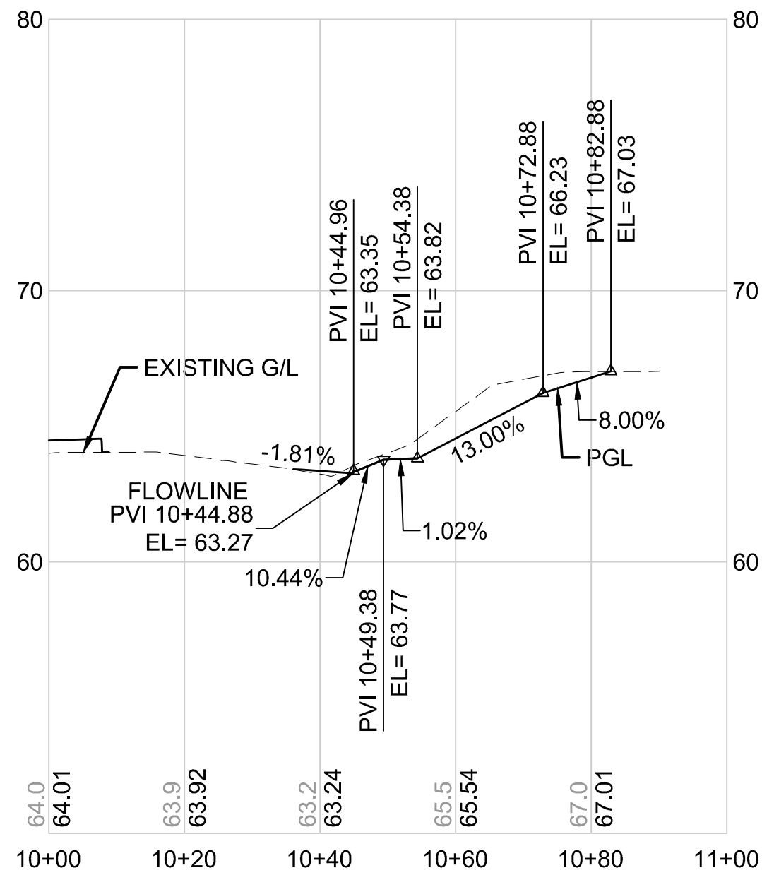
BRS323 LINE HORIZONTAL SCALE: 1"=20' VERTICAL SCALE: 1"=5'
