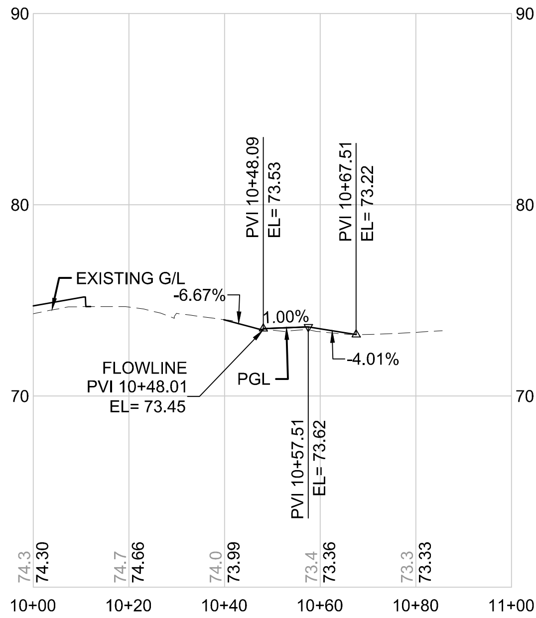
BRS312 LINE HORIZONTAL SCALE: 1"=20' VERTICAL SCALE: 1"=5'
