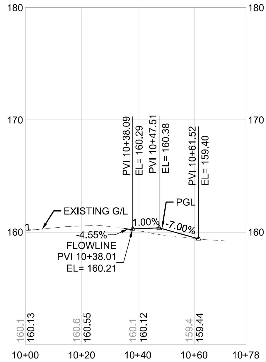
BRS262 LINE HORIZONTAL SCALE: 1"=20' VERTICAL SCALE: 1"=5'
