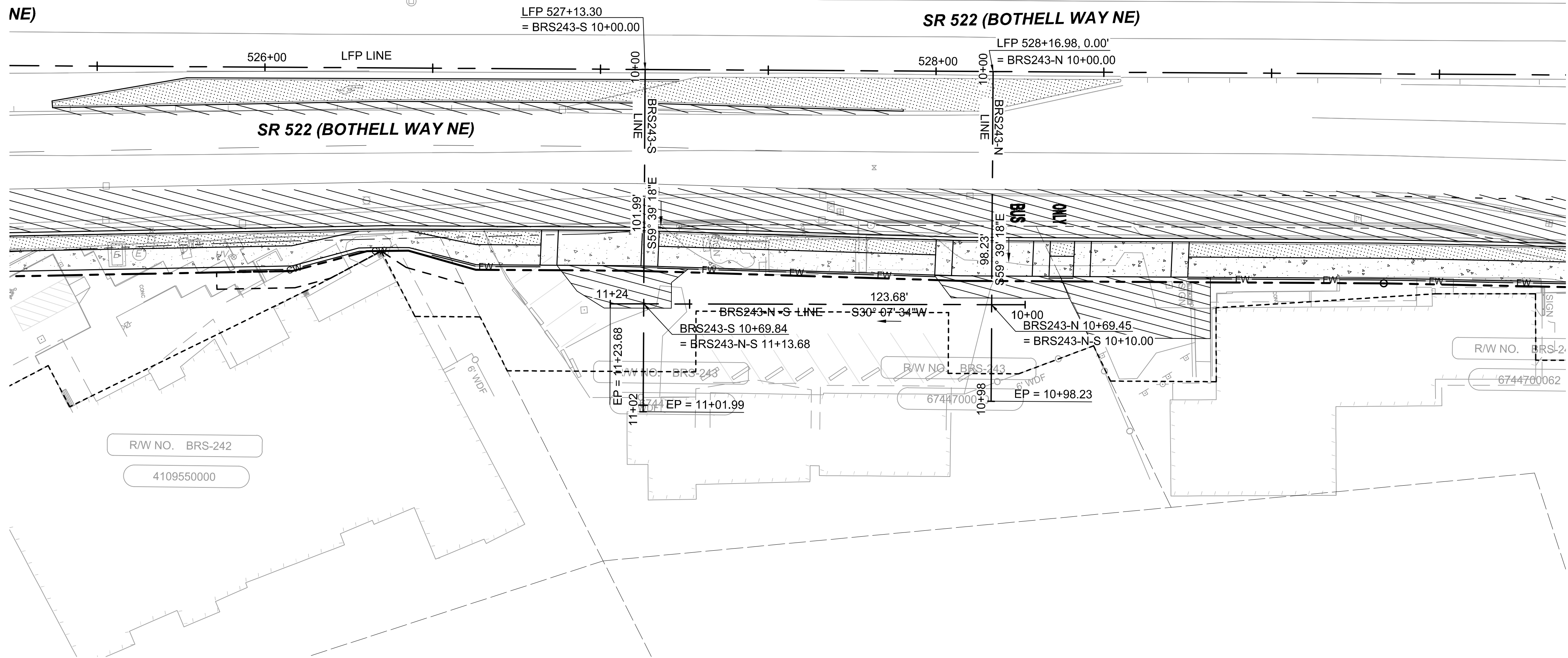
BRS243-S LINE HORIZONTAL SCALE: 1"=20' VERTICAL SCALE: 1"=5'
