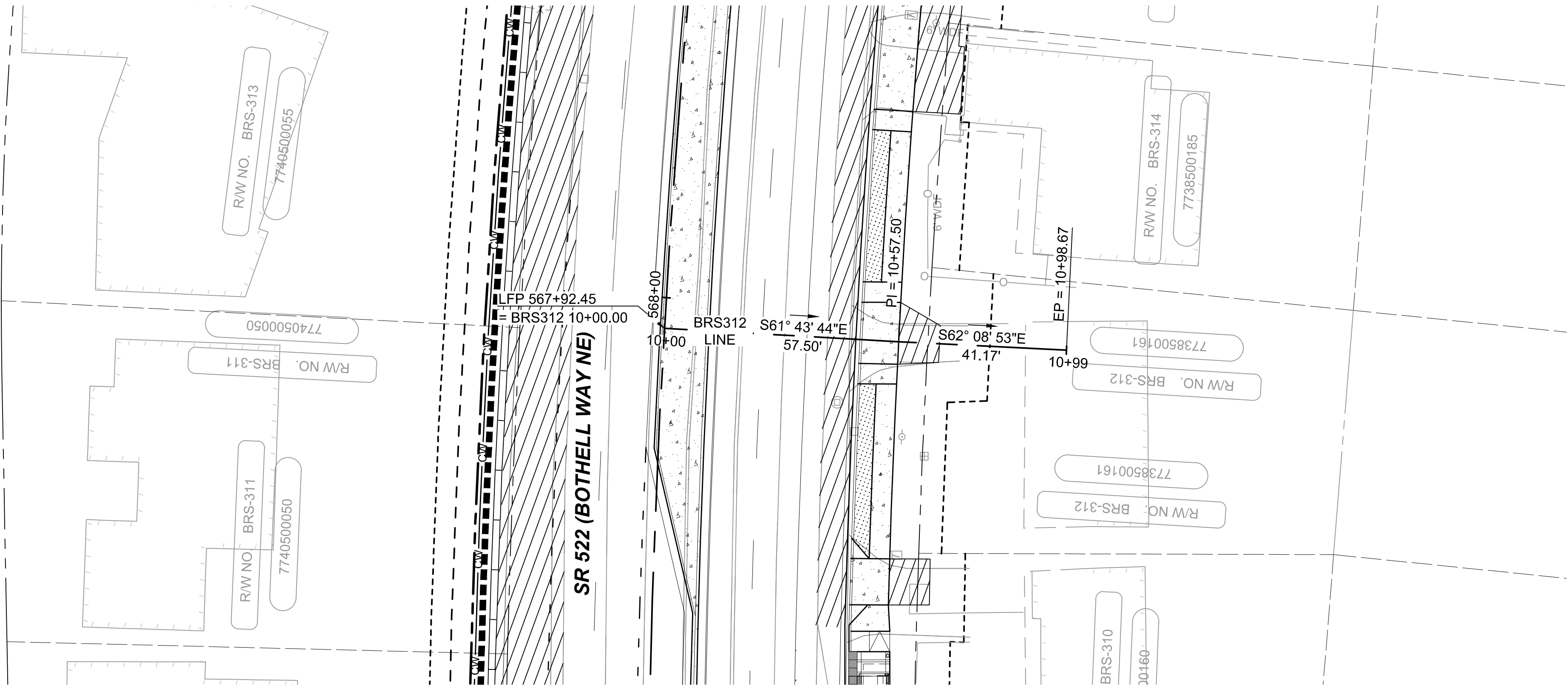
BRS312 LINE HORIZONTAL SCALE: 1"=20' VERTICAL SCALE: 1"=5'
