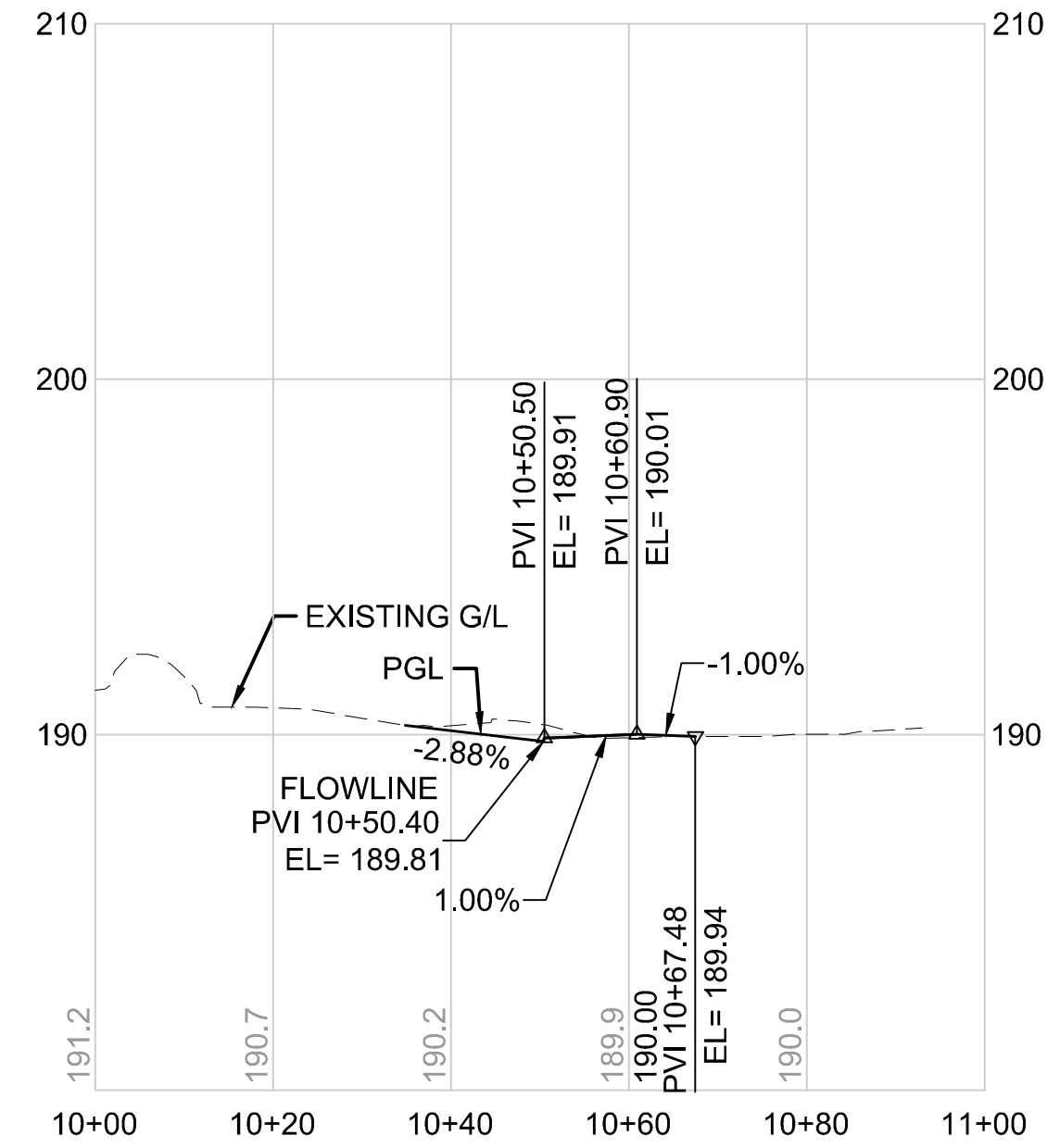
BRS243-N LINE HORIZONTAL SCALE: 1"=20' VERTICAL SCALE: 1"=5'
