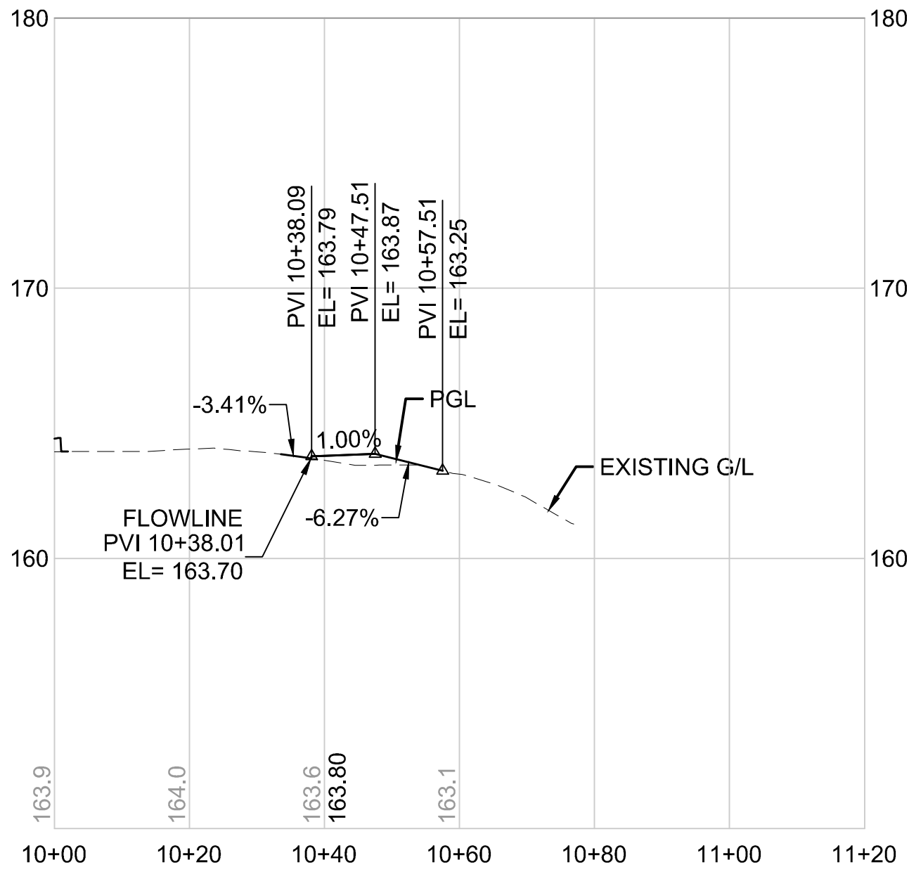
BRS260 LINE HORIZONTAL SCALE: 1"=20' VERTICAL SCALE: 1"=5'
