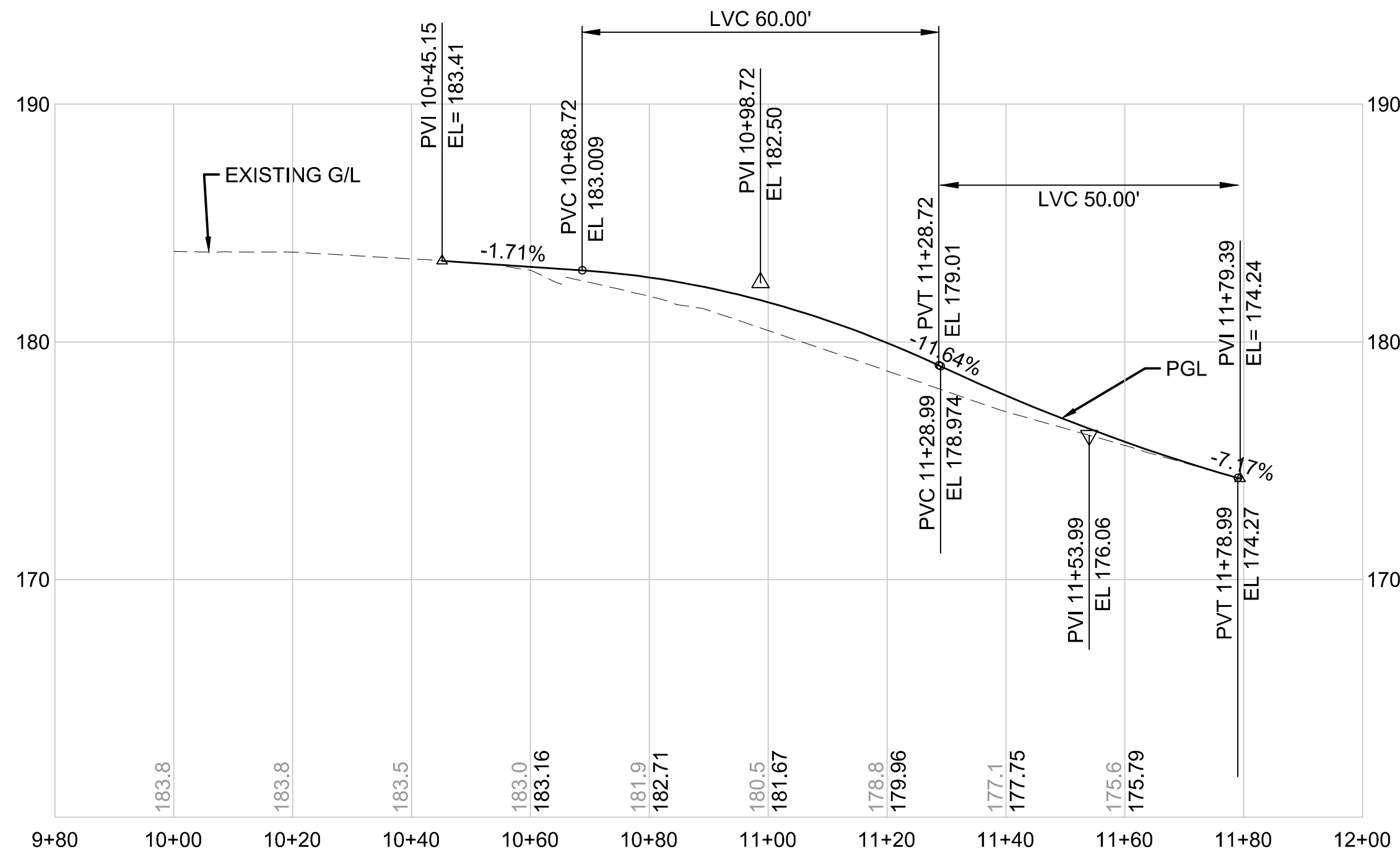
153RD LINE HORIZONTAL SCALE: 1"=20' VERTICAL SCALE: 1"=5'
