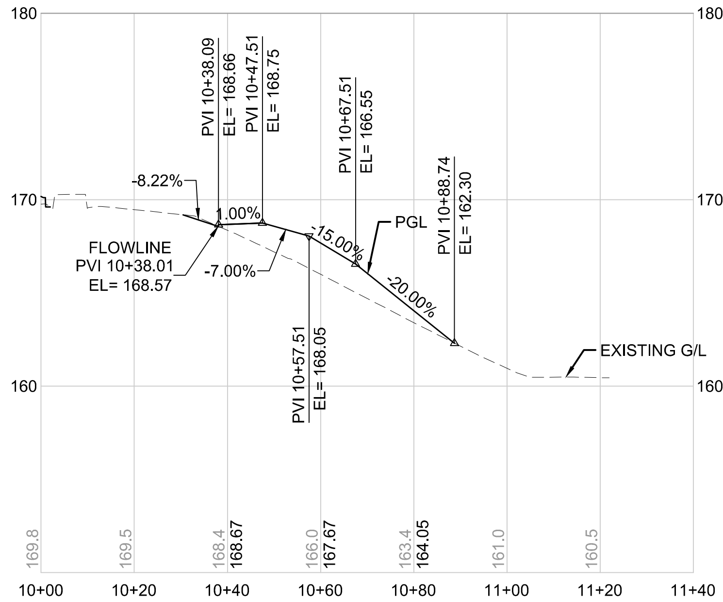
BRS258-S LINE HORIZONTAL SCALE: 1"=20' VERTICAL SCALE: 1"=5'
