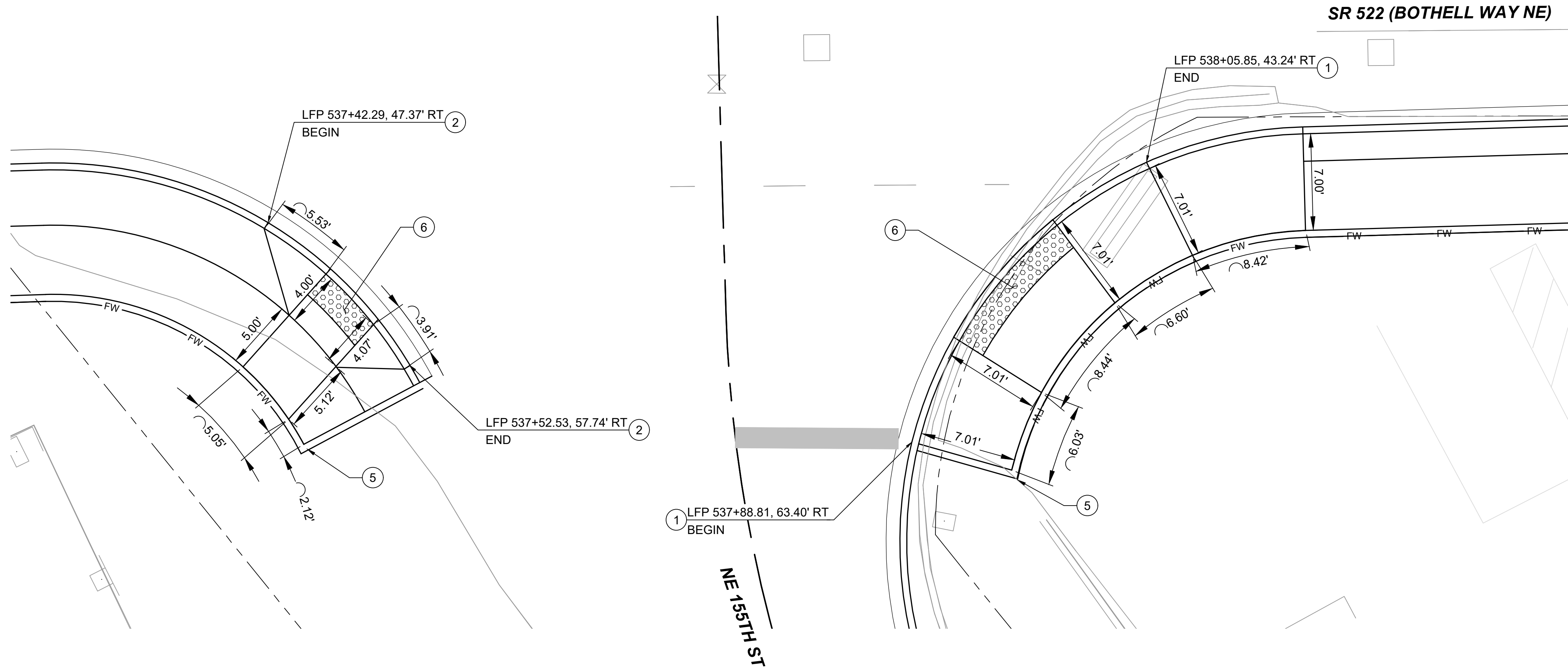
CURB RAMP DETAIL SCALE: 1" = 5'
