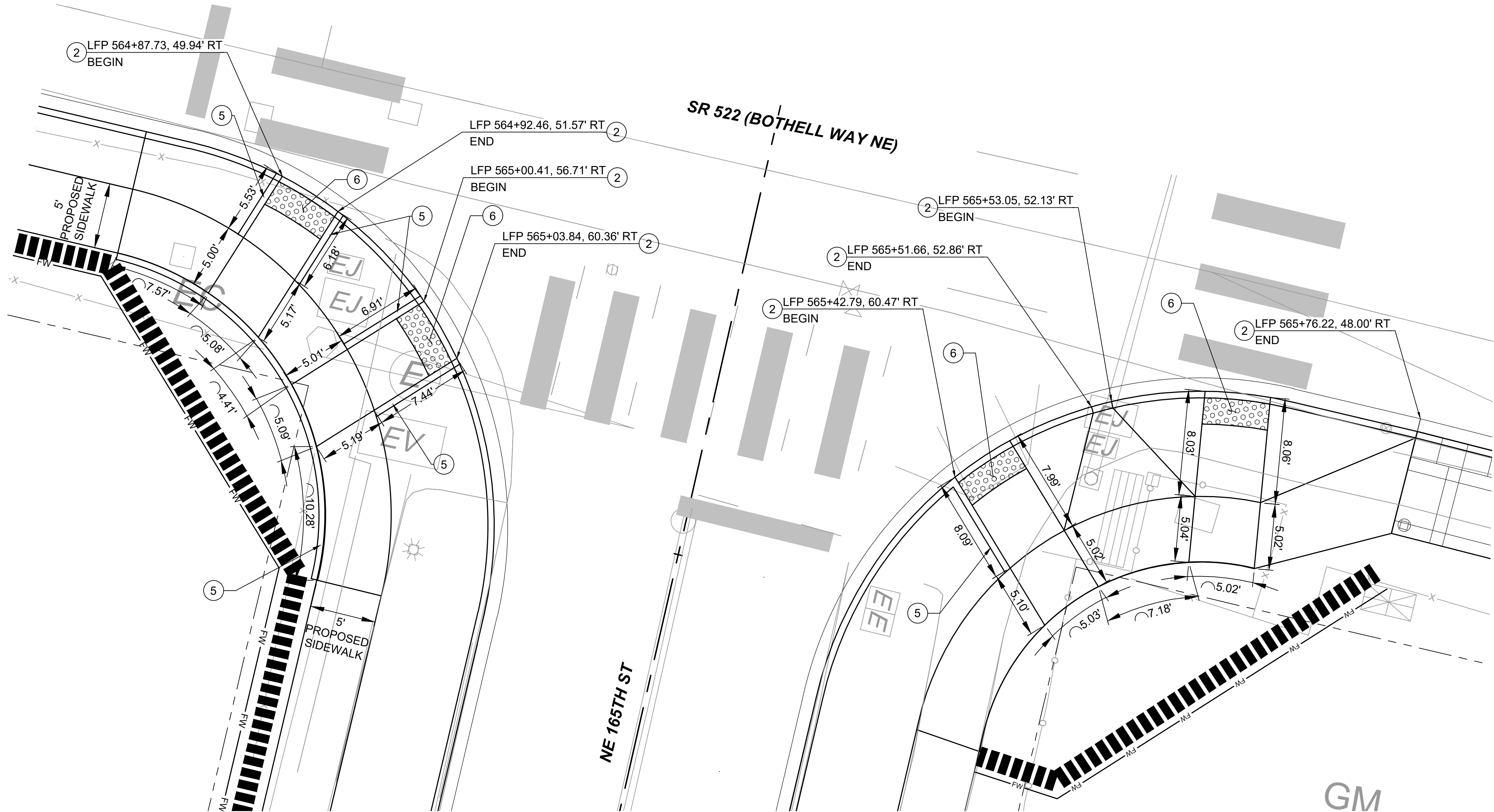
CURB RAMP DETAIL SCALE: 1" = 5'
