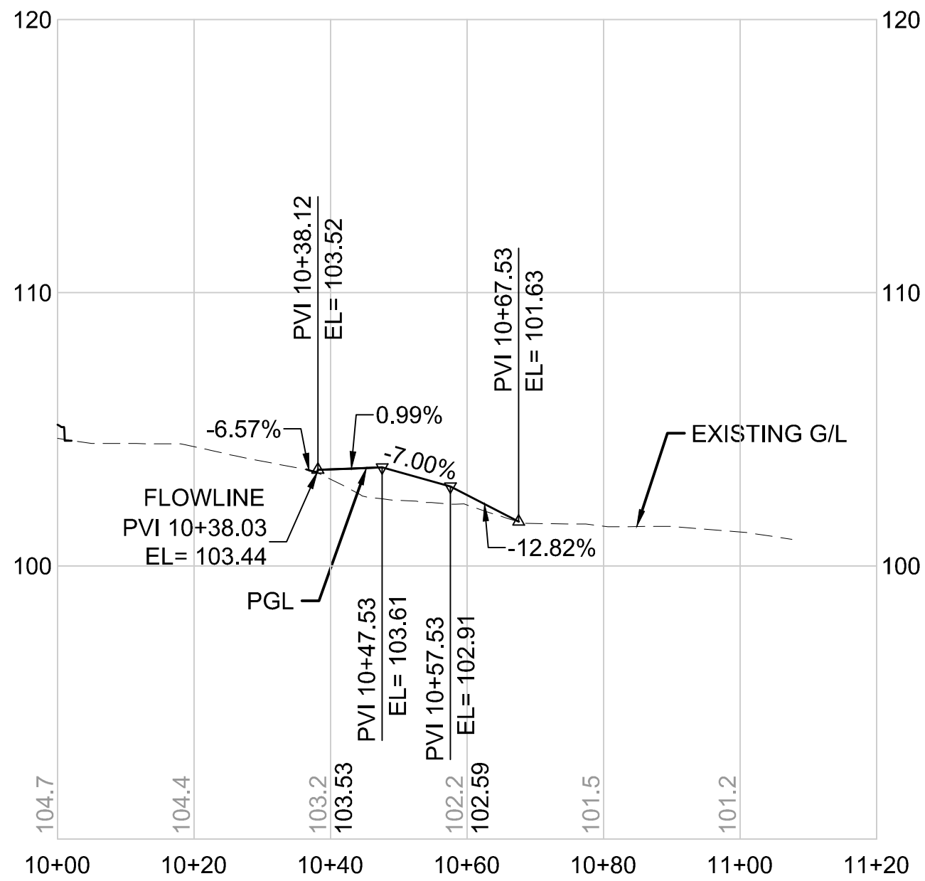
BRS287 LINE HORIZONTAL SCALE: 1"=20' VERTICAL SCALE: 1"=5'
