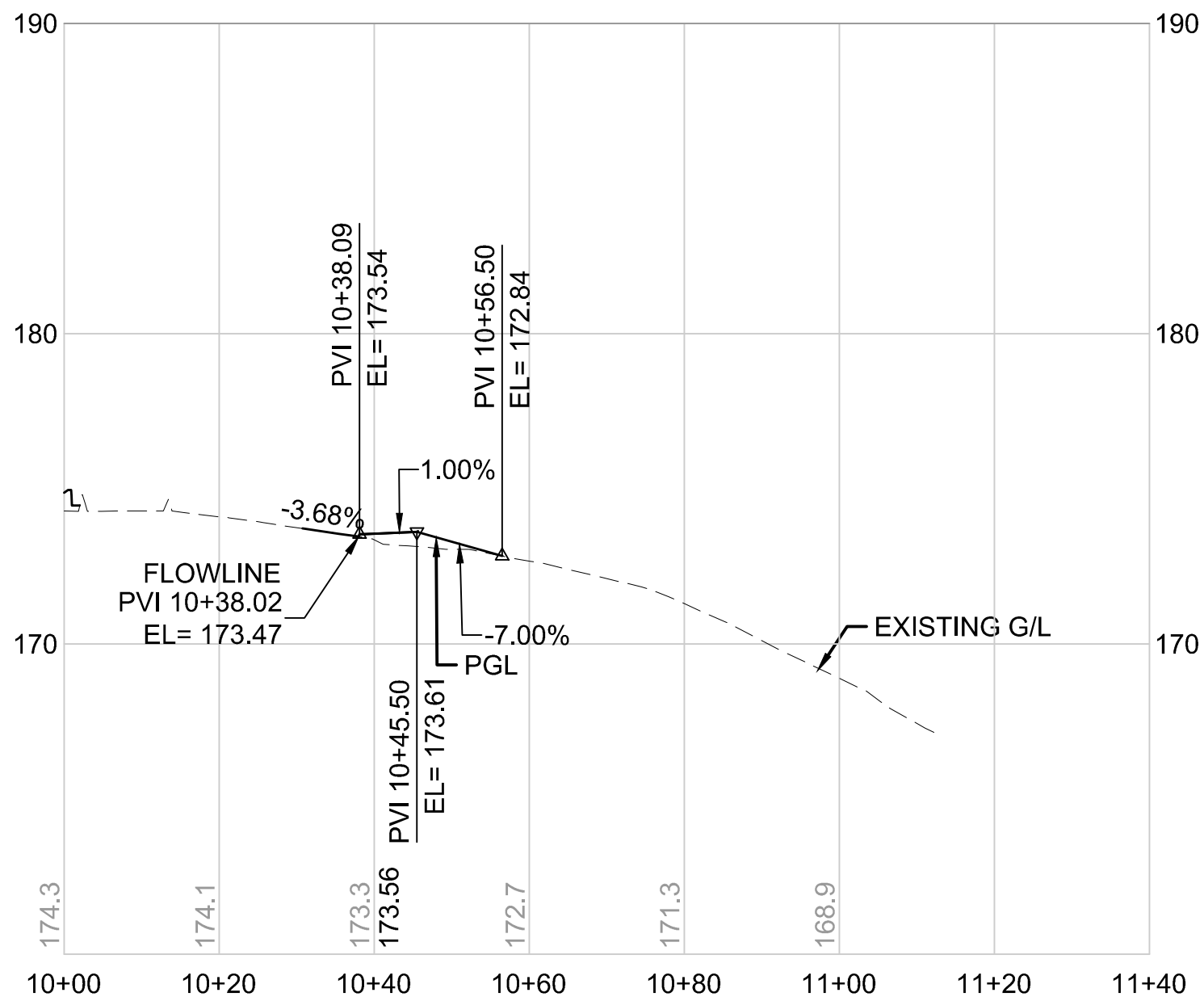
BRS255-256 LINE HORIZONTAL SCALE: 1"=20' VERTICAL SCALE: 1"=5'
