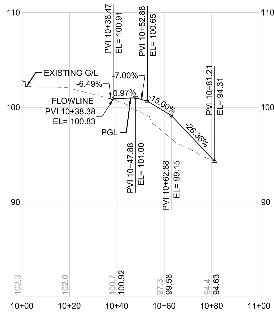
BRS289-S LINE HORIZONTAL SCALE: 1"=20' VERTICAL SCALE: 1"=5'
