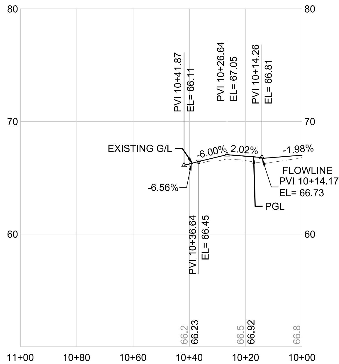
BRS306.1 LINE HORIZONTAL SCALE: 1"=20' VERTICAL SCALE: 1"=5'
