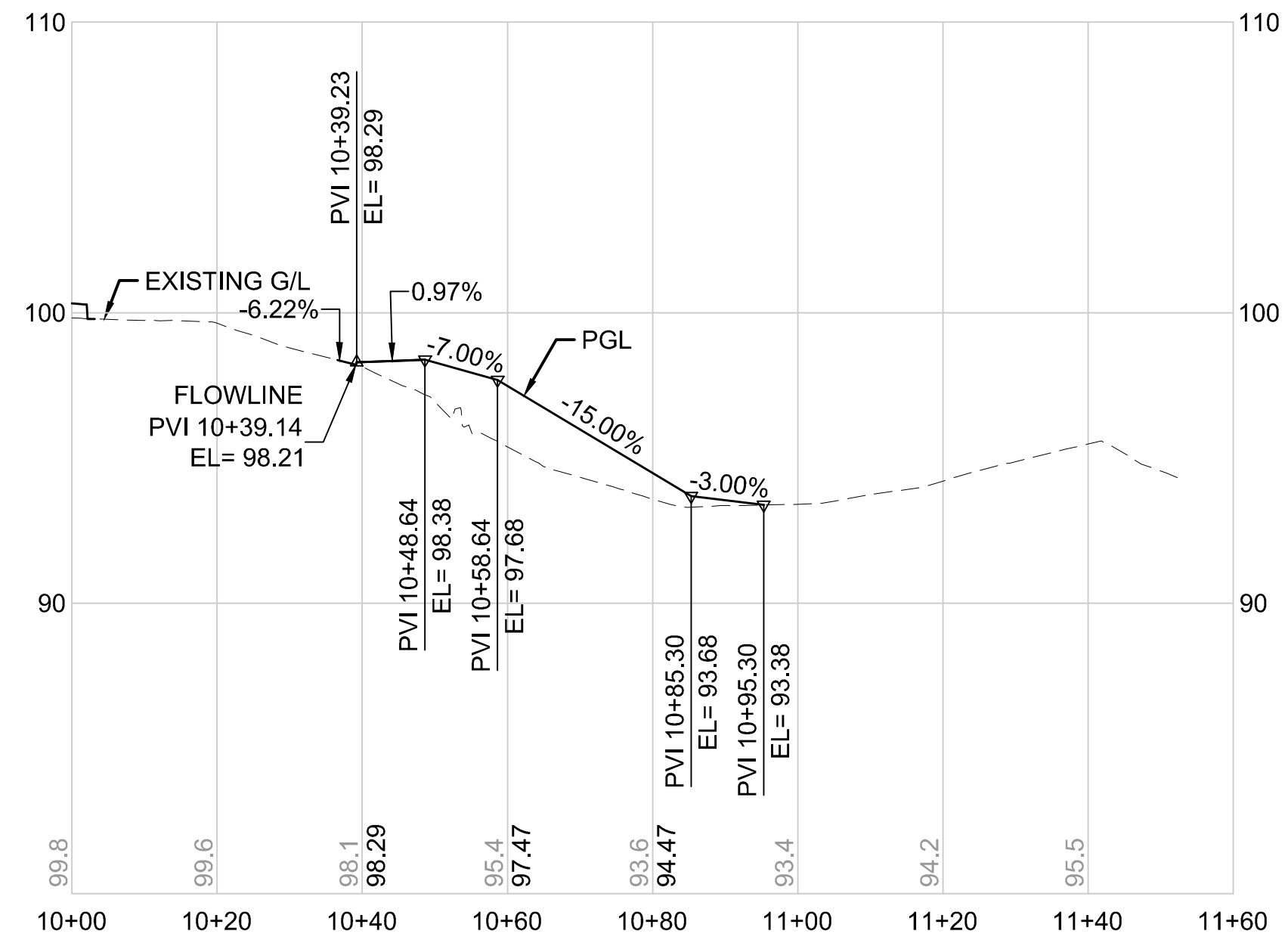
BRS289-N LINE HORIZONTAL SCALE: 1"=20' VERTICAL SCALE: 1"=5'
