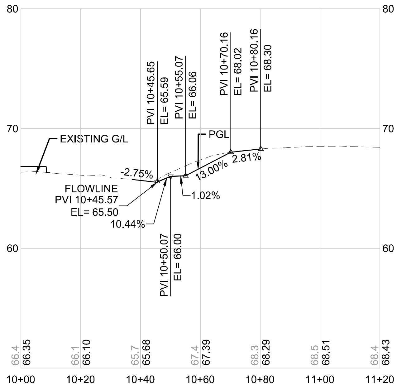
BRS322 LINE HORIZONTAL SCALE: 1"=20' VERTICAL SCALE: 1"=5'
