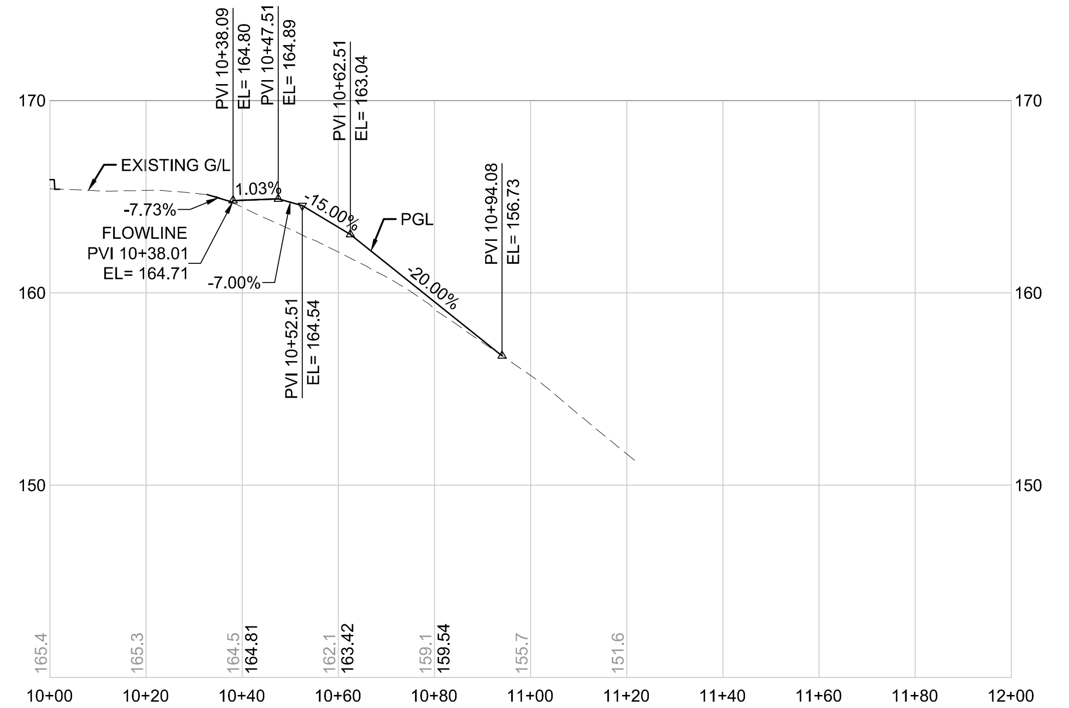
BRS258-N LINE HORIZONTAL SCALE: 1"=20' VERTICAL SCALE: 1"=5'
