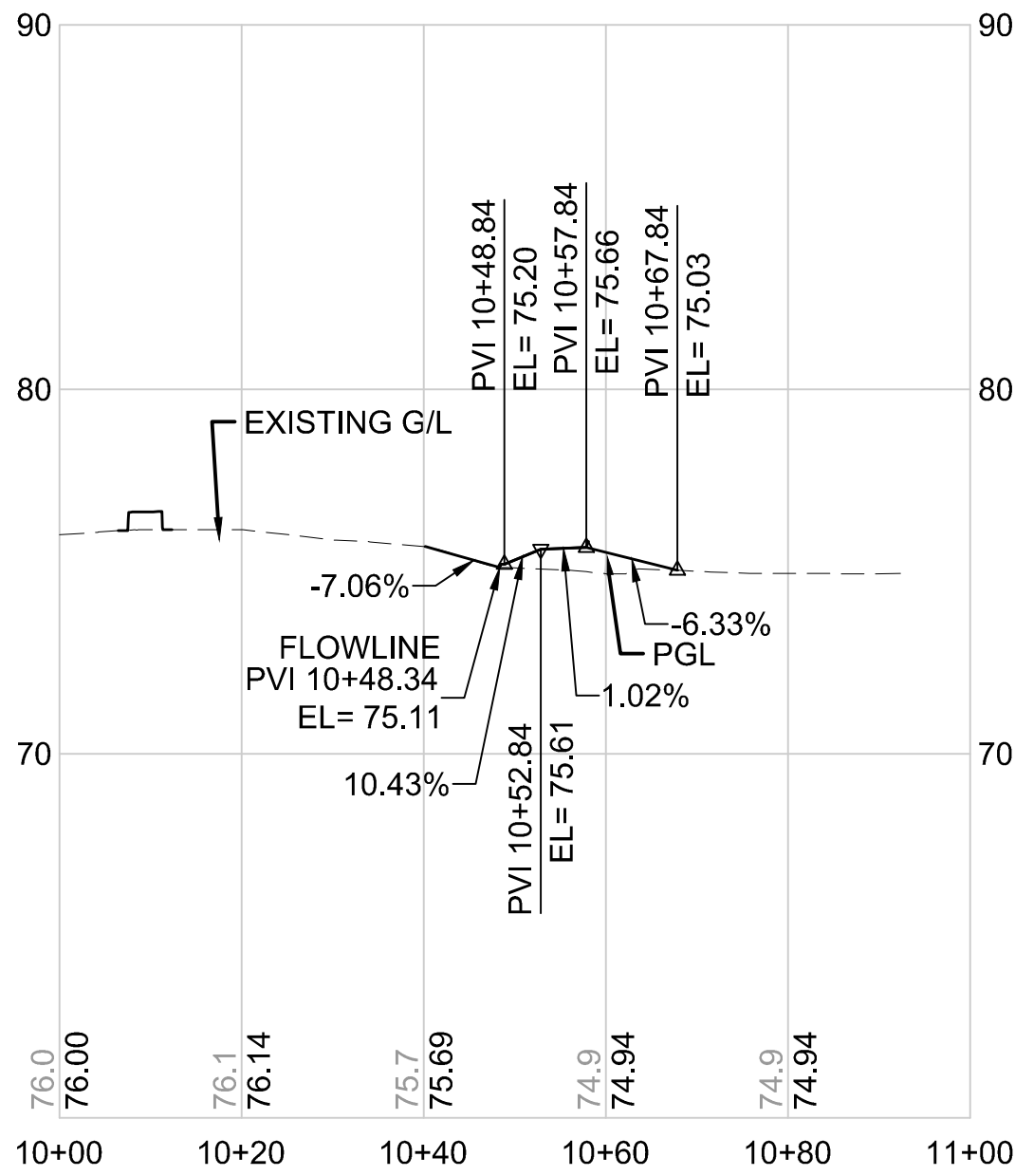
BRS310 LINE HORIZONTAL SCALE: 1"=20' VERTICAL SCALE: 1"=5'
