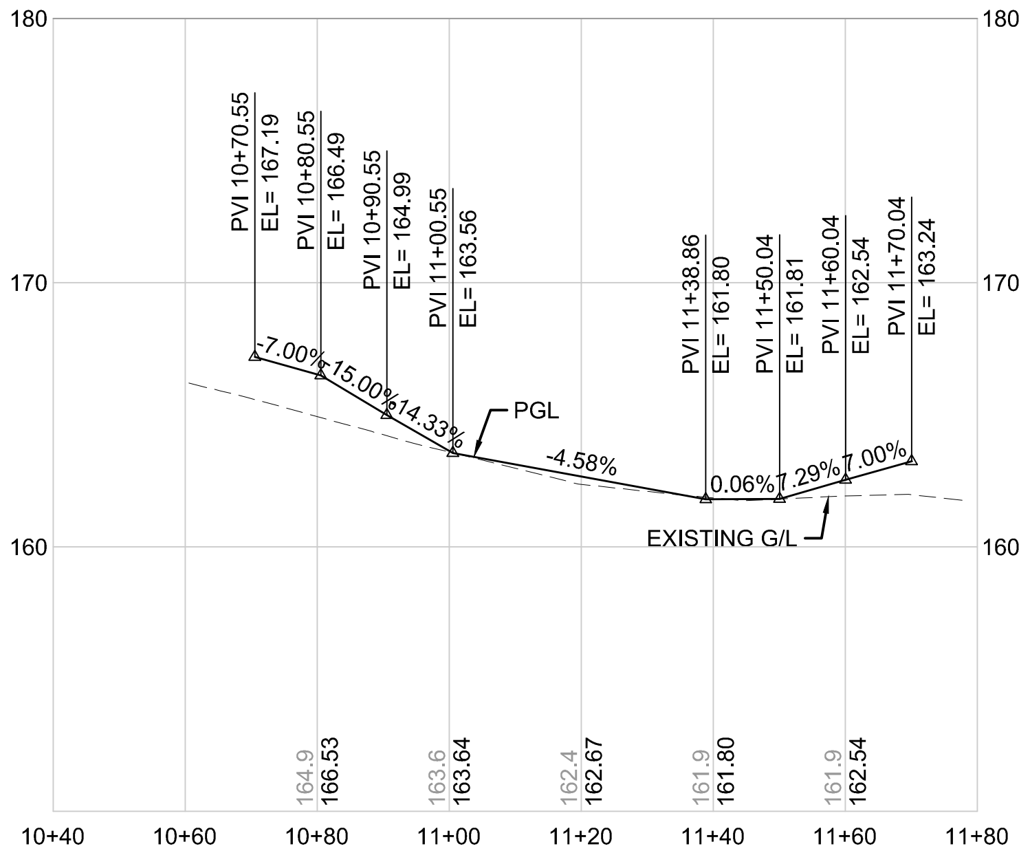
BRS258 N-S LINE HORIZONTAL SCALE: 1"=20' VERTICAL SCALE: 1"=5'
