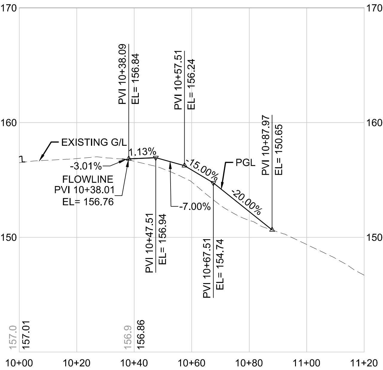
NE 157TH PL LINE HORIZONTAL SCALE: 1"=20' VERTICAL SCALE: 1"=5'
