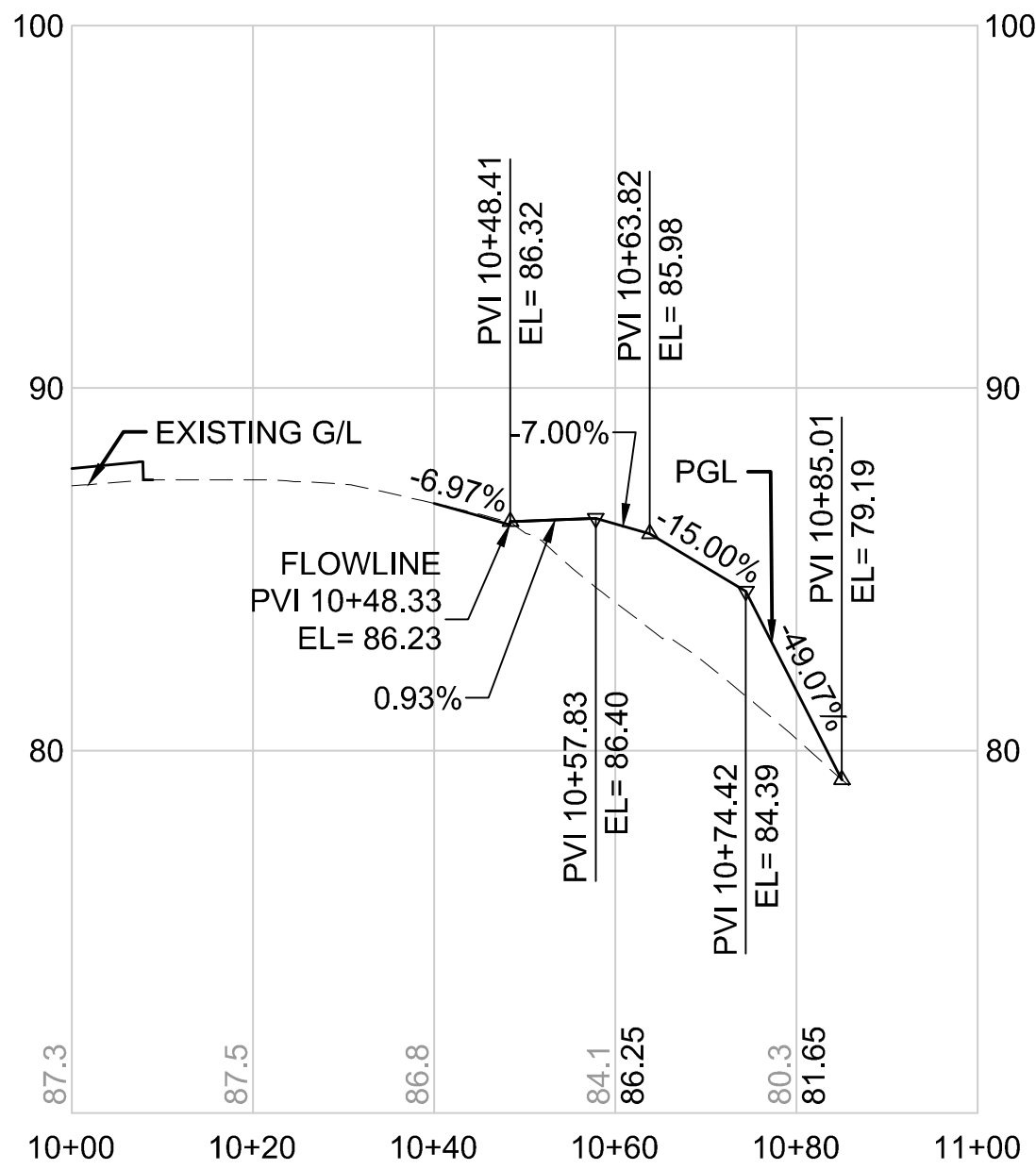
BRS302-S LINE HORIZONTAL SCALE: 1"=20' VERTICAL SCALE: 1"=5'
