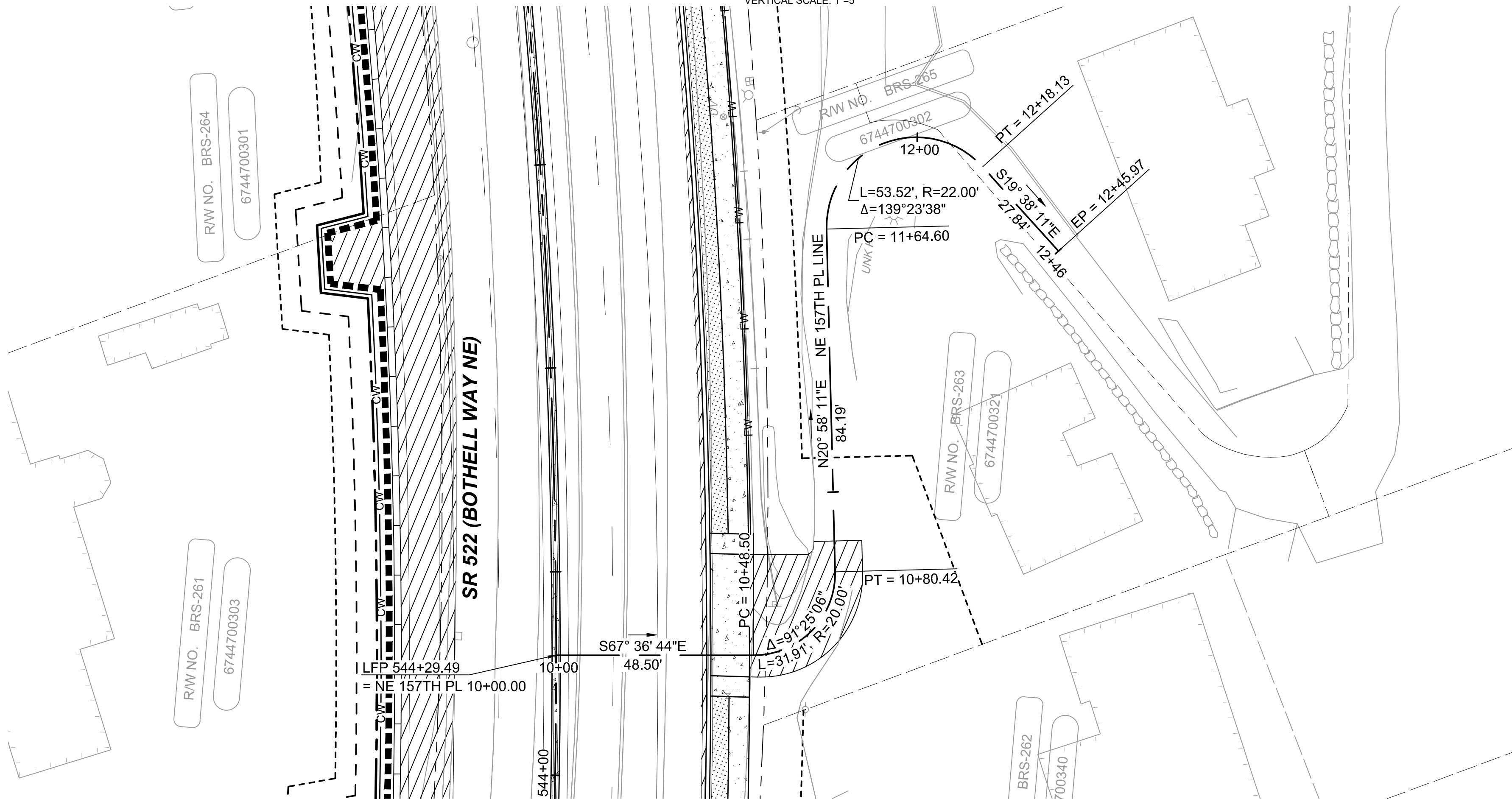
NE 157TH PL LINE HORIZONTAL SCALE: 1"=20' VERTICAL SCALE: 1"=5'
