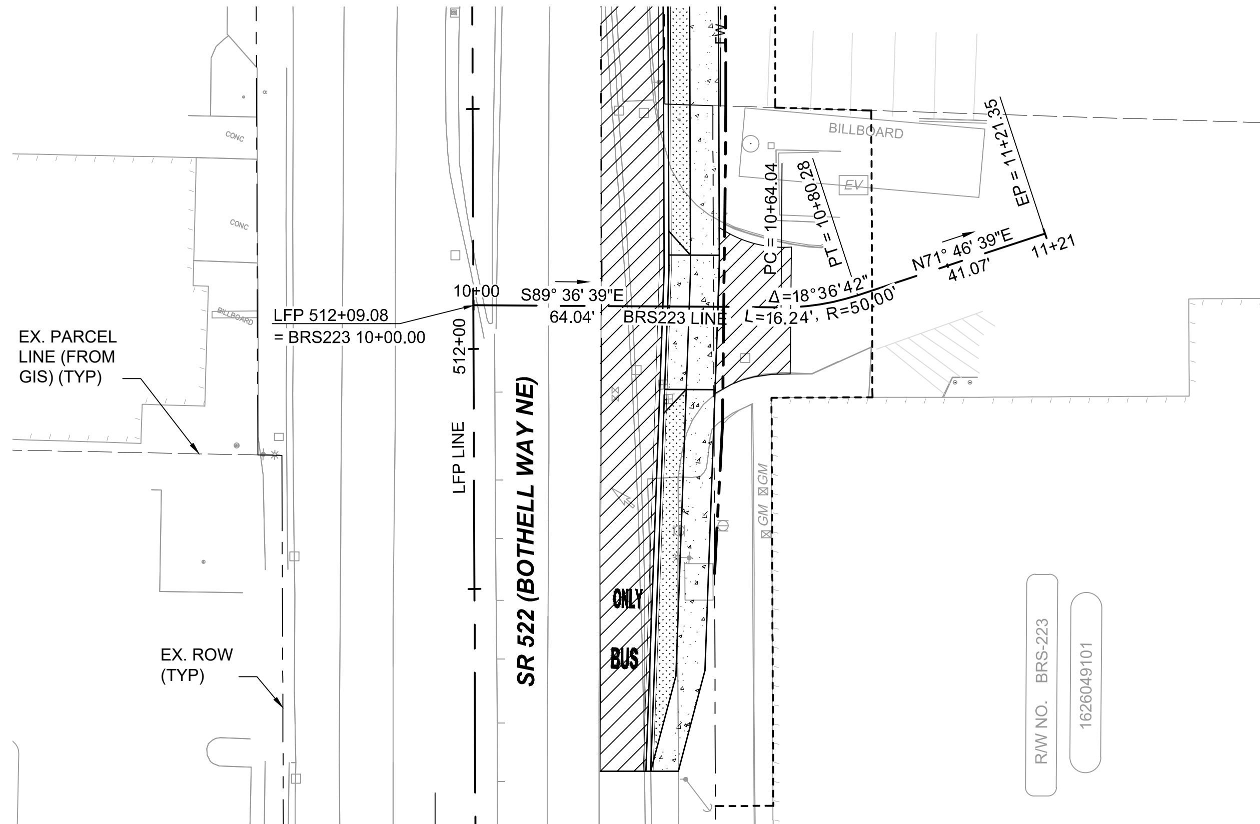
BRS223 LINE HORIZONTAL SCALE: 1"=20' VERTICAL SCALE: 1"=5'
